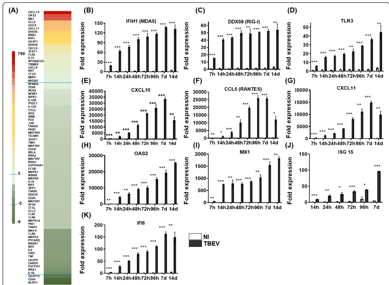
Fig. 5 TBEV-induced antiviral response in hNPC-derived neuronal/glia cells. a TBEV-infected neuronal/glia cells ( MOI 10^{-2} ) and their matched NI controls were analyzed 24 hpi using an RT 2 Profiler PCR array specific for the human antiviral response. The heat map shows the differential expression of 84 analyzed human genes. The most highly up- and downregulated genes are colored in red and dark green, respectively. The blue lines indicate the arbitrary cut-off of 3. Genes between the two lines are considered nonregulated. b–k RT-qPCR analyses of selected antiviral genes. Gene expression was normalized to HPRT1 gene, and the -2\Delta\Delta Ct method was used for relative quantification (normalization to non-infected cells at 7 hpi). Data are expressed as the mean \pm SD. Results are representative of one experiment performed on pooled triplicates (PCR array) or two independent experiments performed in triplicate (qPCRs). Statistical analysis was performed using a two-tailed unpaired t test with Graphpad Prism V6.0.1. ns, non-significant ( p > 0.05 ); * p < 0.05 , ** p < 0.01 , *** p < 0.001
