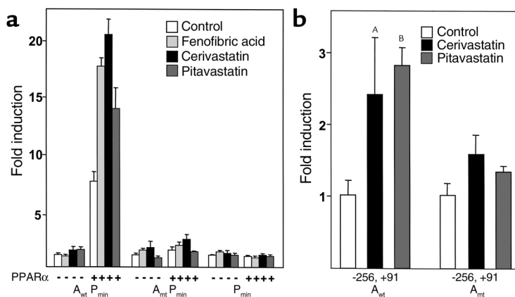
Figure 3 Statins induce human apoA-I A-site activity by PPARα. (a) Reporter plasmids containing the human wild-type and mutated apoA-I A sites cloned upstream of the minimal apoA-I promoter (P min ) (50 ng) were transfected in RK13 cells in the presence of cotransfected human PPARα or empty pSG5 vector plasmids (30 ng) with a Renilla luciferase reporter vector as internal control (2 ng). Cells were treated with cerivastatin (5 μM), pitavastatin (5 μM), fenofibric acid (100 μM), or solvent. Firefly luciferase activities were normalized to Renilla control activities. Values (means ± SD, n = 3) are expressed relative to controls. (b) Reporter plasmids containing the wild-type (-256, +91 A wt ) or A-site mutated (-256, +91 A mt ) apoA-I promoter construct in HepG2 cells with a Renilla luciferase reporter vector as internal control (2 ng). Cells were treated with cerivastatin (5 μM), pitavastatin (5 μM), or solvent. Firefly luciferase activities were normalized to Renilla control activities. Values (means ± SD, n = 3) are expressed relative to controls. Statistically significant differences between statin-treated and control groups are indicated (Scheffé: A P < 0.05; B P < 0.01).
