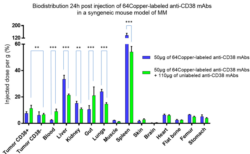
Figure 1. PET-derived biodistribution in a syngeneic model of MM. Tumour-bearing mice were given 50 µg of ^{64}\text{Copper} -labelled anti-CD38 mAbs, associated or not to 110 µg of unlabelled mAbs. With only 50 µg of ^{64}\text{Copper} -labelled anti-CD38 mAbs, modest accumulation was observed in tumours, with no significant uptake differences between CD38– or CD38+ tumours, due to extensive accumulation of the tracer in the spleen. Adding the unlabelled mAbs dose increases tracer availability over time by “saturating” the spleen, allowing for significant increased CD38+ tumour uptake (non-parametric test). Values are expressed in percentage of the injected radioactive dose per gram of tissue and presented as mean \pm SD. **: p -value \leq 0.01 ; ***: p -value \leq 0.001 .
