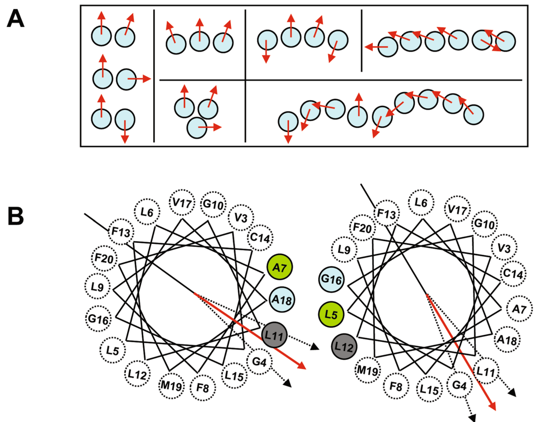
Figure 5. Oligomer formation observed by coarse-grained molecular dynamics simulations of TM24 peptides in DOPC lipids. (A) Topology of the main oligomers observed in the three simulations, as seen from the top. The red arrow within each circle indicates an arbitrary axis in the middle of the TM24 helix enabling to indicate the rotational orientation of each monomer and allowing to distinguish between parallel, orthogonal and symmetrical dimers. (B) Helical wheels representing the most frequent mutual orientation of monomers in dimer (parallel), as seen from the top. Its monomer-monomer interface involves Ala7, Leu11, Ala18 and Leu5, Leu12, Gly16 from each monomer, respectively. Dotted arrows illustrate the angular fluctuation observed both for one dimer along the simulations and between the different dimers within this parallel arrangement.
