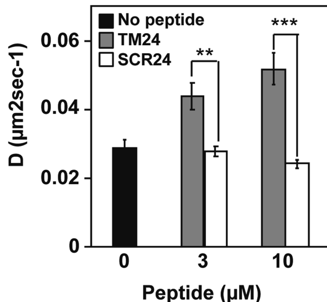
Figure 7. Diffusion rate in cellular membrane of the CX3CL1 protein in the presence of TM24 and SCR24 peptides. The lateral diffusion rate of the CX3CL1-EYFP protein was assayed after transient expression in COS-7 cell line after 15 min preincubation in the presence or not of 3 or 10 μM of TM24 or SCR24 peptides. Each point is the mean of triplicates ± SD.
