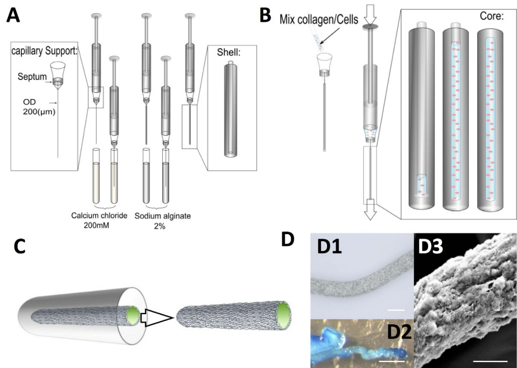
Figure 1. Fabrication procedure of the core-shell fibres. (A) Production of the shell using successive alginate coatings. (B) Production of the core by the substitution of the capillary with collagen/cell suspension. (C) Ability to separate the core from the shell after 24 h of culture. (D1) Representative contrast phase microscopy of a fibre at day 4 (scale = 150 µm). (D2) Representative coloration with methyl blue of a fibre at day 4 (scale = 500 µm). (D3) Representative scanning Electron Microscopy of a fibre at day 4 (scale = 50 µm).
