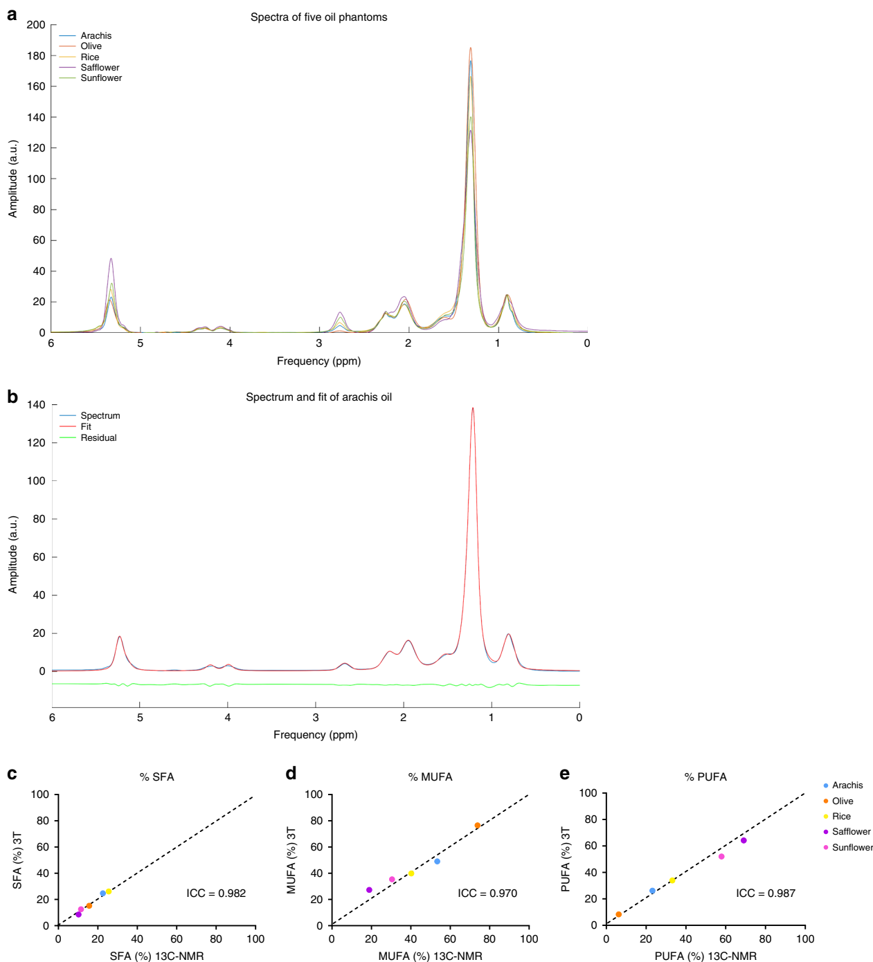
Fig. 1 Validation of 1 H-MRS method in oil phantoms. a Lipid spectra acquired from five different oil phantoms (arachis, olive, rice, safflower, and sunflower oil) showing the different lipid proton peaks and their position. b Lipid spectrum and fit of arachis oil. Correlations between c SFA, d MUFA, e PUFA measured at 3T with 1 H-MRS and measured with high-resolution 13 C-NMR spectroscopy. The intraclass correlation coefficient (ICC) is shown in the respective plots (Intraclass correlation).
