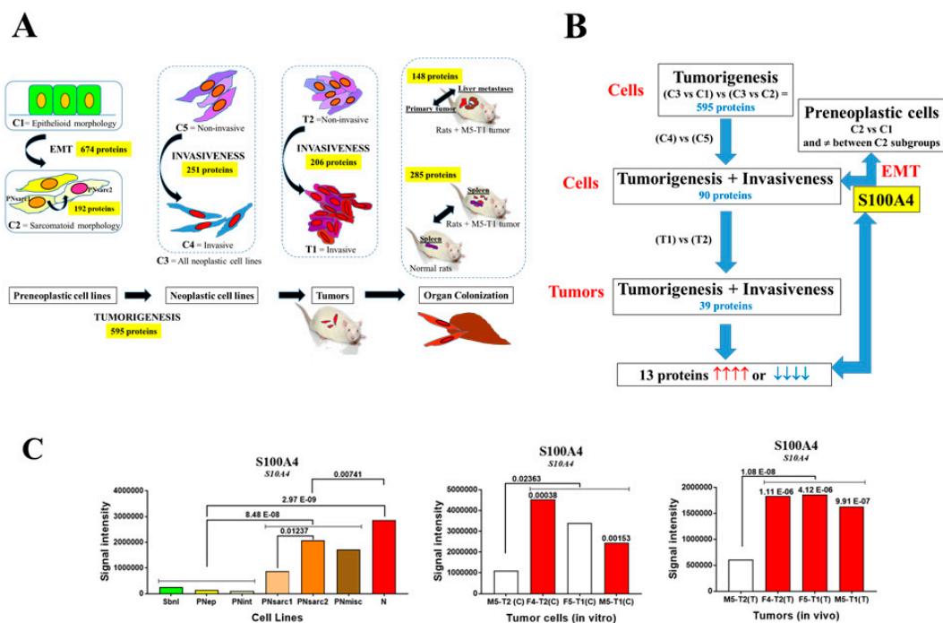
Figure 1. Identification of S100A4 as the main biomarker. (A) Scheme of the successive steps and sources of data used for the identification of candidate biomarkers. C1, preneoplastic cell lines with epithelioid morphology. C2, preneoplastic cell lines with sarcomatoid morphology. C3, neoplastic cell lines. C4, invasive neoplastic cell lines. C5, non-invasive neoplastic cell line. T1, invasive MM (malignant mesothelioma) tumors. T2, non-invasive MM tumor. (B) Methodology used for SWATH-MS (sequential window acquisition of all theoretical fragmentation spectra) proteomic analyses of cell lines and tumors. (C) Comparative proteomic abundances of S100A4 (significant increases in red and decreases in blue, with p values). Left: comparison between the different subgroups and groups of preneoplastic and neoplastic cell lines (in vitro); middle: comparison between invasive and non-invasive neoplastic cell lines (in vitro); right: comparison between invasive and non-invasive mesotheliomas (in vivo). Blank bars correspond to the absence of significant differences between cell lines/tumors.
