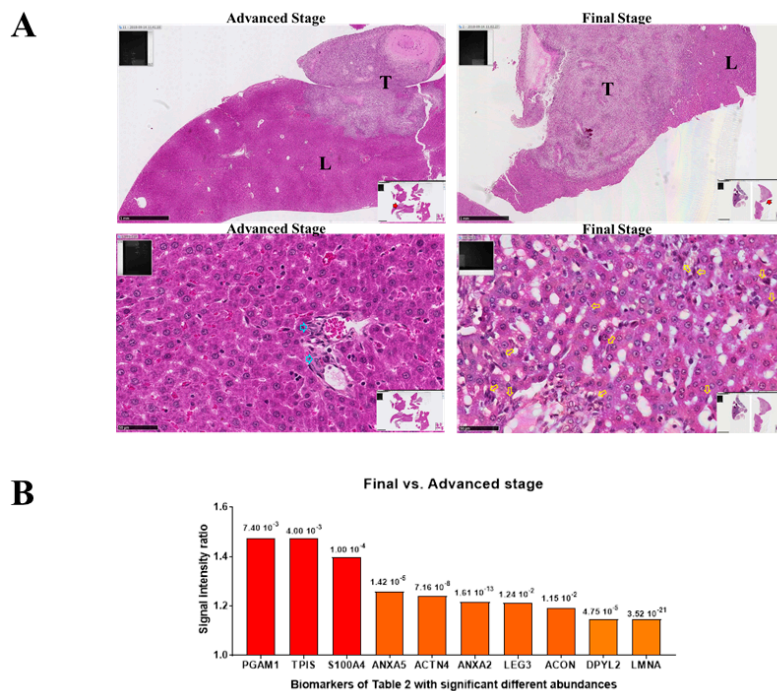
Figure 4. Comparison between liver metastases and primary tumor, M5-T1 tumor model. (A) Histological features of the two stages identified in the colonization of the liver by M5-T1 cells. Top rank, general views ( \times 25 , the scale bar represents 1 mm) showing the extent of tumor (T) development within the liver tissue (L). Bottom rank, detailed views ( \times 400 , the scale bar represents 50 \mu\text{m} ). The final stage was characterized by the presence of numerous isolated metastatic M5-T1 cells infiltrating the liver parenchyma (yellow arrows), in contrast to the advanced stage for which the tumor cells were only localized within the portal triad (blue arrows). (B) Proteomic analysis: Abundance ratios (final versus advanced stage) for the 11 biomarkers exhibiting significant differences ( p < 0.05 ), and also found in the list of 39 biomarkers detailed in Table 2, p values are indicated for each biomarker at the top of the bars.
