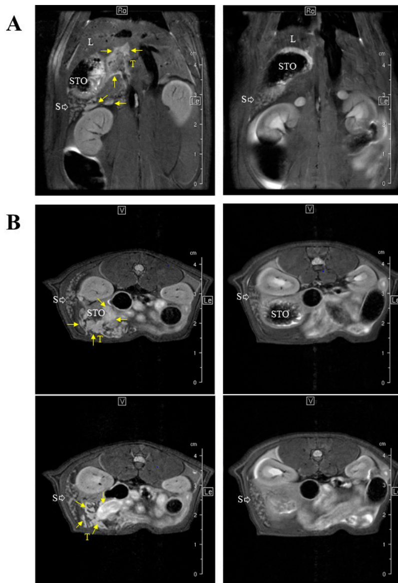
Figure 3. MRI-based staging of the M5-T1 MM model. M5-T1 tumor (T, and yellow arrows) was present as omental cakes and nodules attached to the stomach (STO) and spleen (S) on both coronal (A) and axial images (B). M5-T1 tumor was also characterized by the presence of metastatic tumor development into the liver parenchyma (L) and along the portal vein. Note the changes in volume and white pulp vs. red pulp signal intensity of the spleen in the tumor-bearing rat in comparison to normal rat spleen.
