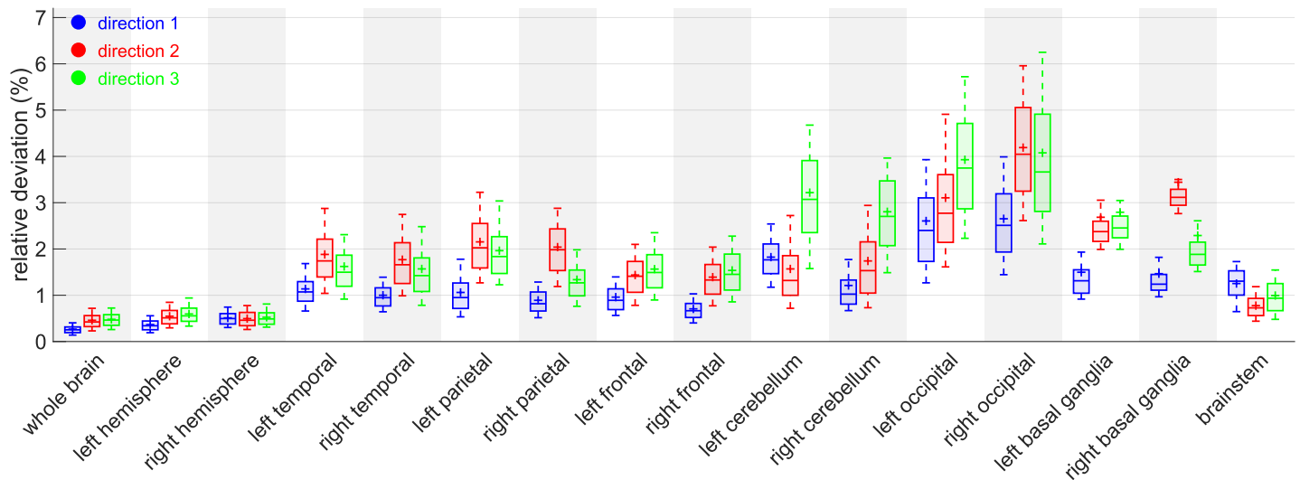
Fig 17. Relative standard deviation between reference atlases. Boxplots among subjects for each ROI j , each direction d : \text{boxplot}(D(\cdot, j, d)) .
