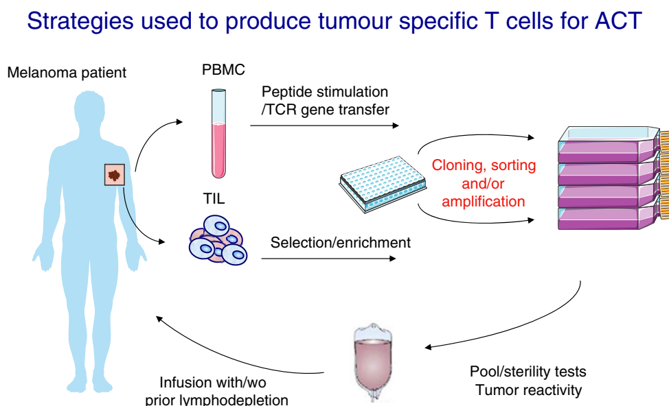
Fig. 1 The production of autologous tumor-specific T cells for a use in ACT trials can be achieved either from TIL (spontaneously enriched in tumor-specific T cells) or PBMC. PBMC are enriched in antigen-specific T cells, either by peptide stimulation or TCR gene transfer. TIL populations can be also enriched in antigen-specific T cells by additional steps of selection (based on tumor reactivity or antigen specificity). Thereafter, tumor specific T cells can be sorted or cloned and/or in vitro expanded. After the final expansion step, T cells are pooled and tested for sterility and tumor reactivity, just before their transfer to the autologous patients
