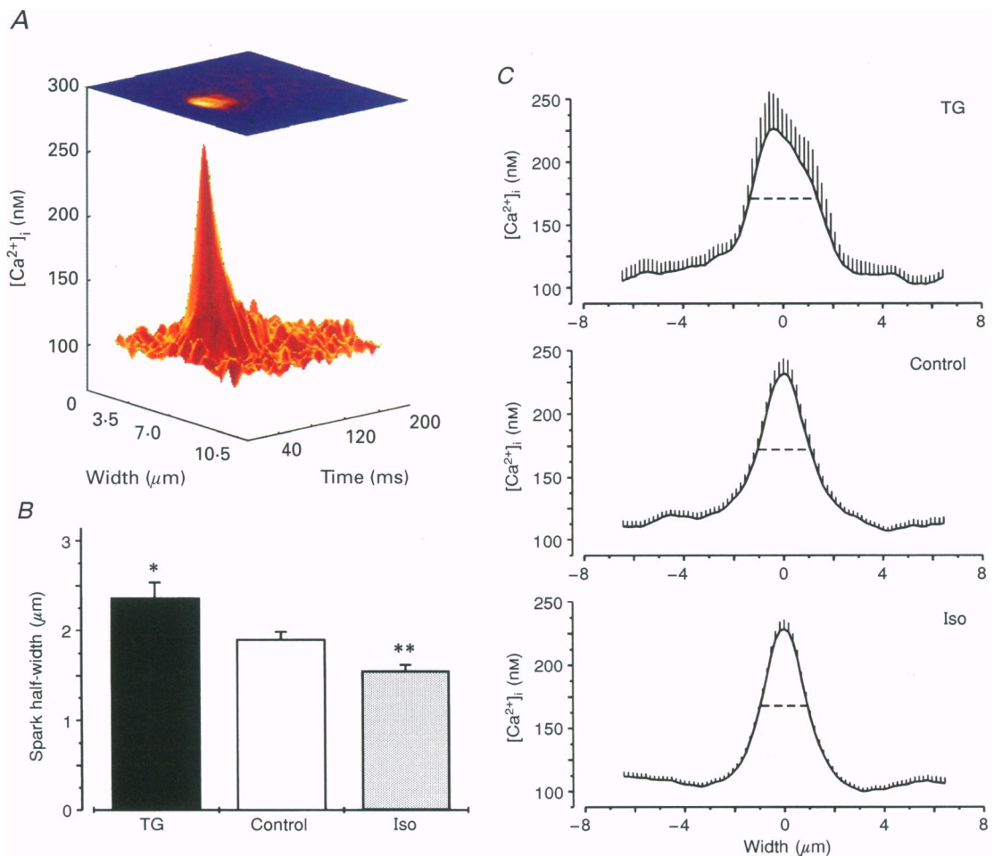
Figure 3. Spatial spread of Ca 2+ sparks after SR Ca 2+ pump blockade or stimulation
