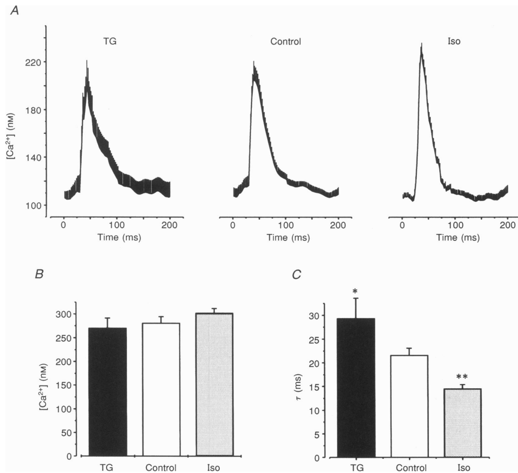
Figure 2. \text{Ca}^{2+} spark characteristics after SR \text{Ca}^{2+} pump blockade or stimulation
