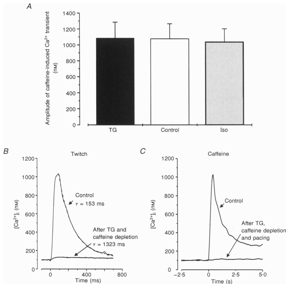
Figure 1. SR Ca 2+ content and twitch [Ca 2+ ] i transients before and after thapsigargin
