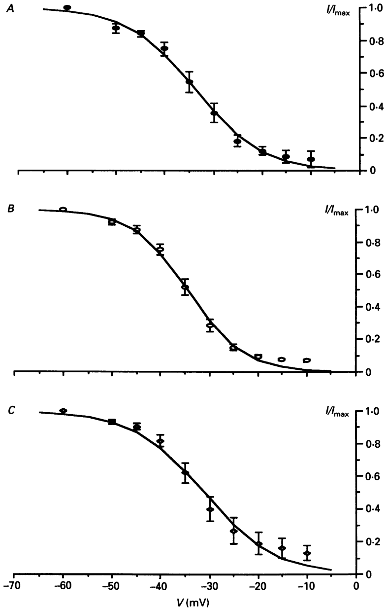
Fig. 7. Steady-state inactivation-voltage relationships of I_{to} in hypertrophied septum ( A ), apex ( B ) and left ventricular free wall ( C ) myocytes. The smooth curves were fitted to the mean data points using a Boltzmann distribution as described in text. Vertical bars represent \pm s.e.m.
