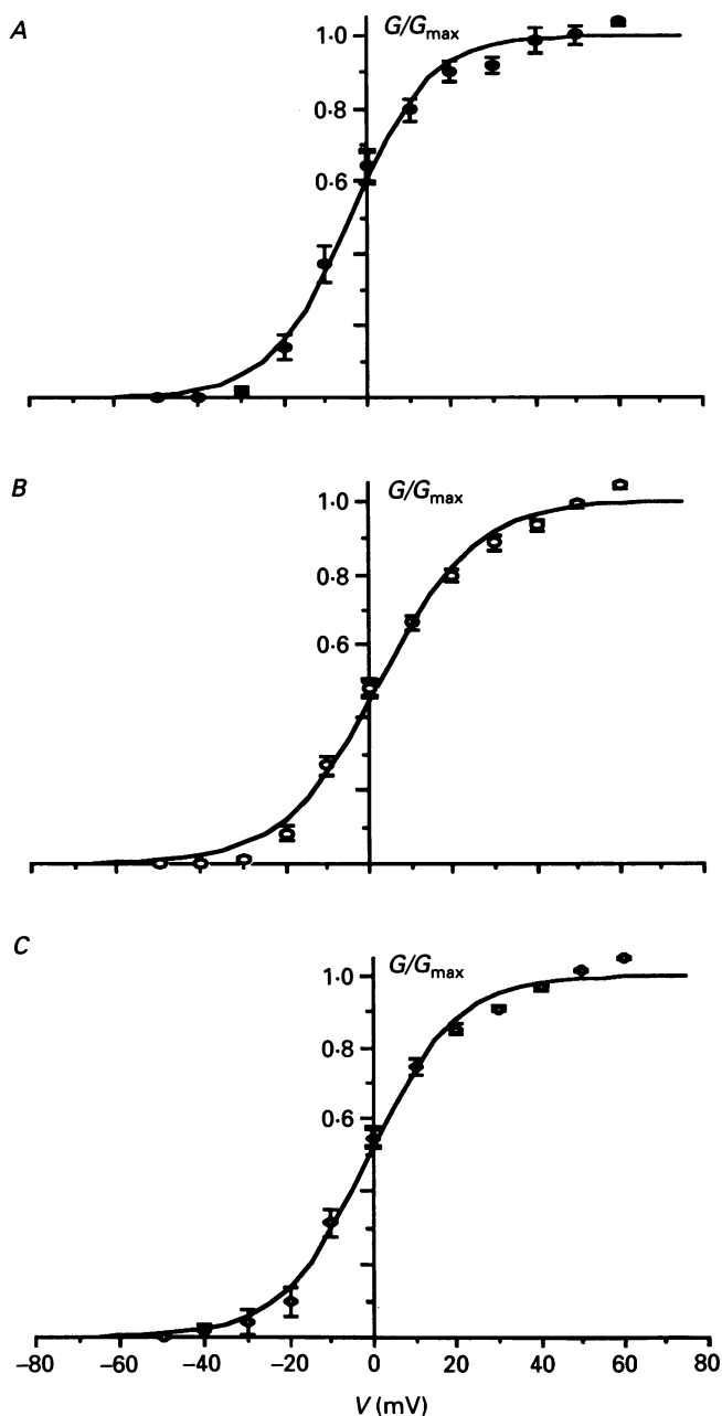
Fig. 8. Steady-state activation-voltage relationships of I_{to} in hypertrophied rat ventricular myocytes. Normalized mean chord conductance in septum (A), apex (B) and left ventricular free wall (C) myocytes were plotted versus membrane potential. The curves were fitted through the mean data points according to the procedure described in the text. Vertical bars represent \pm s.e.m.
