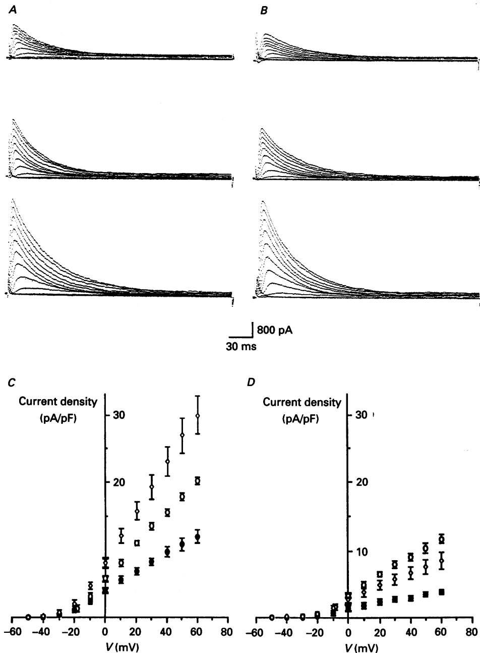
Fig. 2. Current-voltage relationships for I_{to} . A and B , representative current traces of I_{to} in normal ( A ) and in hypertrophied ( B ) myocytes isolated from septum (top traces), apex (middle traces) and left ventricular free wall (bottom traces). Current traces were obtained by subtraction of records in the presence of 4-AP from those in control conditions induced by 300 ms depolarizing pulses (0.2 Hz) from a holding potential of -80 mV to test voltages ranging from -50 to +60 mV (from lowest to highest traces, in 10 mV increments; currents were filtered at 10 kHz and digitized at sample intervals of 600 \mu s). C and D , mean current density-voltage relationships of I_{to} : C , in normal
