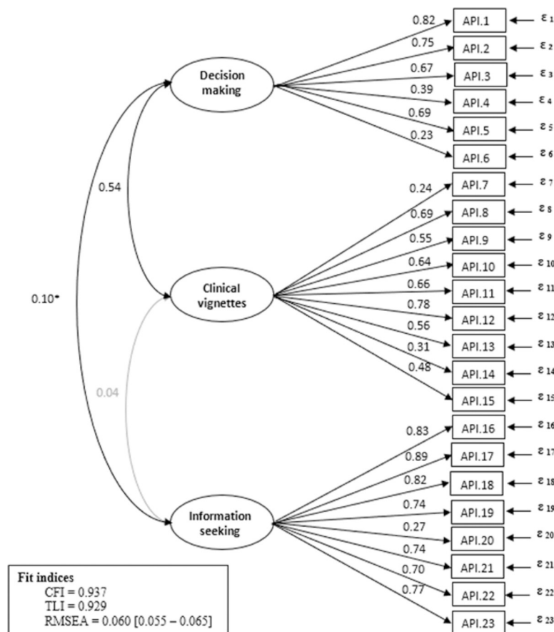
Fig 1. Path diagrams (with standardized coefficients) for the three factor model with fit indices using a confirmatory factor analysis (robust weighted least squares [WLSMV] estimator). Ellipses represent unobserved latent factors, rectangles represent observed variables, single-headed arrows represent the effect of one variable on another (factor loading) and double-headed arrows represent covariance between pairs of variables. Coefficients are all statistically significant with a p -value < 0.001 , except * p -value = 0.039 and coefficient in grey which is not statistically significant. \epsilon : measurement error df: degree of freedom. CFI: Comparative Fit Index. TLI: Tucker Lewis Index. RMSEA: Root Mean Square Error Approximation.
