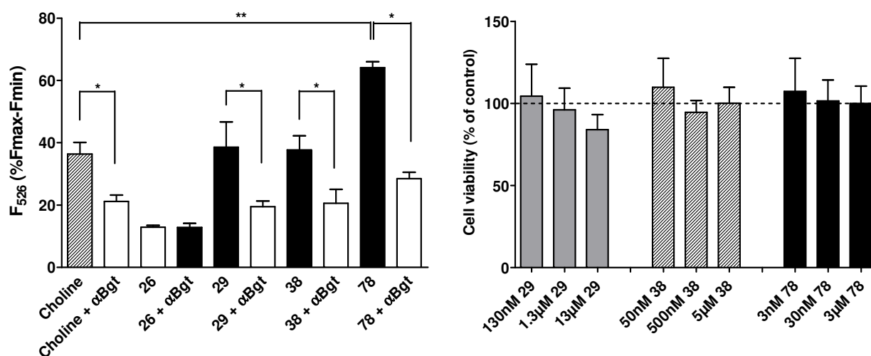
Figure 3. Panel A: Intracellular calcium release in human SH-SY5Y cells expressing native \alpha 7R. Cells were loaded with fluo-3 AM and preincubated with 100 nM \alpha -bungarotoxin ( \alpha -Bgt) for 20 min and PNU-120596 for 1 min before stimulation with 3 mM choline or molecules 26 (7 nM), 29 (130 nM), 38 (50 nM) and 78 (3 nM), as described in the Materials and Methods. In order to normalize fluo-3 AM signals (excitation \lambda Ex = 506 nm, emission \lambda Em = 526 nm), the maximum and minimum fluorescence from each well was determined by addition of 0.3% Triton-X100 (F max ) followed by 100 mM MnCl 2 (F min ). Drug-evoked responses were expressed as a percentage of the corresponding (F max -F min ) value. Fluorescence was recorded in a Varioskan Flash spectral scanning multimode reader. Results are the mean \pm SEM of 5 independent experiments in duplicate. Panel B: Cell viability. SH-SY5Y cells were incubated during 48 hours with increasing concentrations (10 Ki, 100 Ki and 1000 Ki) of molecules 29 , 38 and 78 . The MTS reagent was added and the reading of the optical density of the formazan was carried out after 3 hours of incubation using the Varioskan Flash spectral scanning multimode reader (490 nm). The results are expressed as
