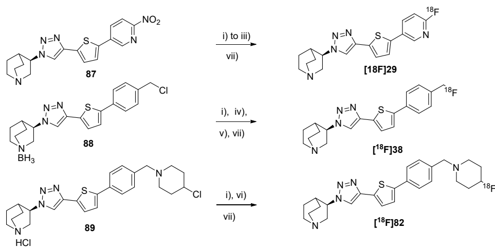
Scheme 5. Nucleophilic radiosynthesis of potent compounds with ^{18}\text{F} starting from their corresponding precursors. Reagents and conditions: i) [ ^{18}\text{F} ]KF / \text{K}_{2.2.2} , DMSO, 150 °C, 10
