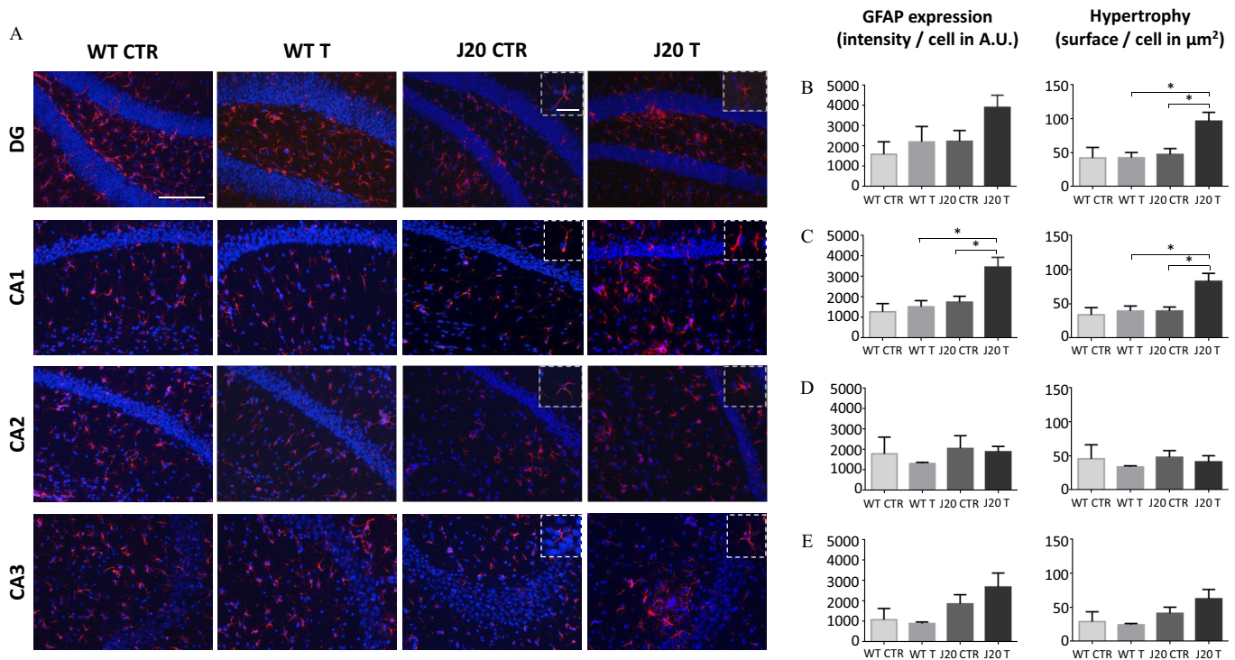
Figure 4. (A) Astrocyte labeling in the hippocampus of WT and J20 mice treated with the fungicide cocktail or with DMSO for 9 months and (B) quantification of GFAP expression and hypertrophy of astrocytes in the dentate gyrus (DG), (C) CA1, (D) CA2, and (E) CA3 areas. (A) Representative images of brain tissue sections labeled with an anti-GFAP antibody to visualize astrocytes. Brain tissue sections from WT and J20 mice, either treated with the cocktail of fungicides (0.1 \mu\text{g}/\text{L} each) (T) or with an equivalent volume of DMSO ( 3 \times 10^{-5}\% ) (CTR) for 9 months were used to quantify the intensity (astrogliosis) and the surface area (hypertrophy) of the GFAP labeling. Results were normalized by the total number of cells. These parameters were quantified on 8–10 hippocampus per animal, for the DG (B), the CA1 (C), the CA2 (D), and the CA3 (E) areas. Values are expressed as mean \pm SEM and a two-way ANOVA followed by a Holm-Sidak's post hoc analysis was used to evaluate statistical differences ( \alpha = 0.05 , ^*p < 0.05 ). Scale bar: 100 \mu\text{m} (magnification \times 20 ). Inserts are representative images of the astrocyte status in the different groups (scale bar: 50 \mu\text{m} , magnification \times 40 ). n = 3\text{--}4 animals per group issued from Study 2. Note: A.U., arbitrary units; ANOVA, analysis of variance; CTR, control; DMSO, dimethyl sulfoxide; GFAP, glial fibrillary acidic protein; T, treatment; WT, wild type.
