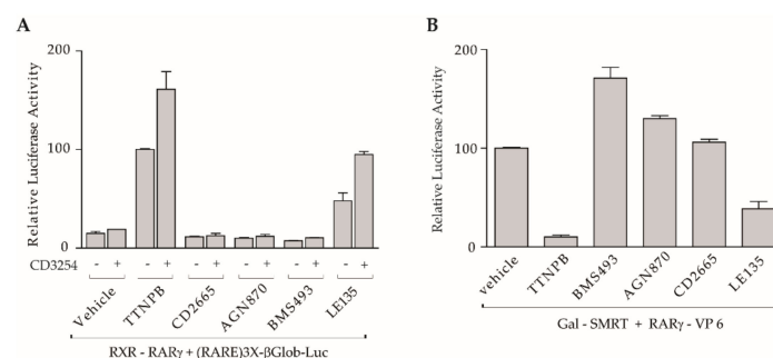
Figure 4. CD2665 and AGN870 do not synergize with CD3254 to activate RXR-RAR \gamma . (A) transient transactivation in COS cells co-transfected with the reporter (RARE)3x-tk-Luc and RAR \gamma and RXR expression vectors in the absence or in the presence of indicated retinoids used alone or with CD3254 (100%, TTNPB induced activity); (B) mammalian two-hybrid assay with (17m)5x- \beta Glob-Luc and VP16-RAR \gamma and Gal-SMRT was performed in COS cells to assess the influence of indicated retinoids on interaction between RAR \gamma and CoRs (100%, basal transcriptional activity). Compounds were used at 1 \mu M in all two-hybrid assays. Error bars, s.e.m.
