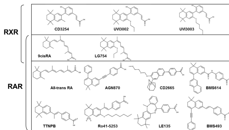
Figure 1. Chemical structures of the retinoids and rexinoids used in this study.
