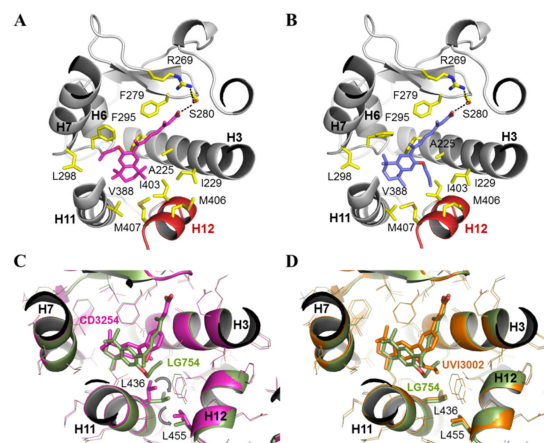
Figure 8. Structural basis of LG754 activity in RAR \beta and RXR \alpha . (A,B) close-up view of LG754 in the LBP of RAR \beta as observed in the two molecules of the asymmetric unit. Side chains of residues in close contact with the ligand are shown as yellow sticks. In both cases, hydrogen bonds between the carboxylate group of LG754, R269 in H5 and S280 in the \beta -turn are highlighted in dashed black line. The propoxy group of the ligand points either toward helices H6 and H7 (in a) or toward helix H12 (in b); (C) close-up view of the superposition of RXR \alpha LBP bound to LG754 (in green, PDB code 6sti) with RXR \alpha LBP bound to CD3254 (in pink, PDB code 3fug) [68]. The propoxy group of LG754 pointing toward H12 induces a reorientation of L436 from helix H11, as compared to its position in the RXR \alpha -CD3254 complex, generating a steric clash with L455 of helix H12; (D) close-up view of the superposition of RXR \alpha LBP bound to LG754 (in green, PDB code 6sti) with RXR \alpha LBP bound to UVI3002 (in orange, PDB code 2p1v) [54]. The aliphatic extension of UVI3002 induces the same positioning of L436 and L455, as observed in the structure of RXR \alpha bound to LG754.
