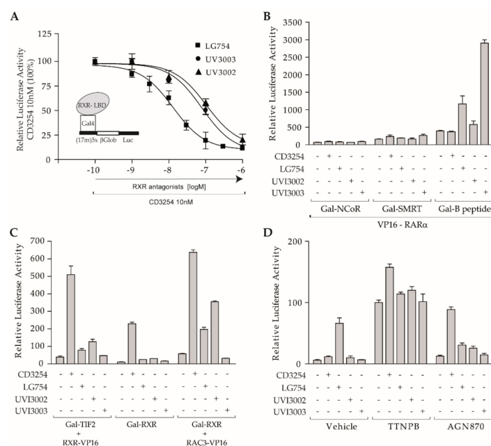
Figure 5. Contribution of different classes of rexinoids in the RXR-RAR \alpha heterodimer activity. (A) To assess antagonistic activities of synthetic rexinoids, COS cells were co-transfected with (17m)5x- \beta Glob-Luc and Gal-RXR expression vector. The reporter was activated by 10 nM CD3254 (100%) and increasing concentrations of LG754 (closed squares) or UVI3002 (closed triangles) or UVI3003 (closed circles) were added in a concentration range of 10^{-10} to 10^{-6} M, as indicated; (B) mammalian two-hybrid assays with (17m)5x- \beta Glob-Luc and VP16-RXR and Gal-NCOR (left panel) or Gal-SMRT (middle panel) or Gal-B peptide were performed in COS cells to assess the influence of indicated retinoids on interaction between RXR and CoRs. Compounds were used at 1 \mu M; (C) mammalian two-hybrid assays with (17m)5x- \beta Glob-Luc and Gal-TIF2 and VP16-RXR (left panel) or with Gal-RXR and RAC3-VP16 (right panel) were performed in COS cells to assess the influence of indicated retinoids on interaction between RXR and TIF2 and to reveal the partial agonist activity of RXR antagonists. Transactivation assay with Gal-RXR used alone is shown in the middle panel. Compounds were used at 1 \mu M; (D) transactivation assays in MRLN cells to assess the activity of the indicated rexinoids on RXR-RAR \alpha activity when used alone or in association with either TTNPB or AGN870 (100%, TTNPB induced activity). Compounds were used at 1 \mu M. Error bars, s.e.m.
