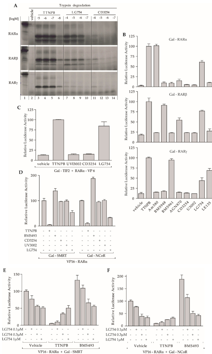
Figure 6. LG754 is a partial agonist for all three RARs. (A) RAR protease sensitivity reveals LG754 binding to RARs. Partial proteolysis maps of in vitro-translated RARs in the presence or the absence either of TTNPB, LG754, or CD3254 at the indicated concentrations. Radiolabeled RARs were exposed to trypsin for 10 min. (Top) RAR \alpha , (Middle) RAR \beta , (Bottom) RAR \gamma ; (B) COS cells were transiently co-transfected with the reporter (17m)5x- \beta Glob-Luc and Gal-RAR \alpha (Top), Gal-RAR \beta (Middle) or Gal-RAR \gamma (Bottom), as indicated, to assess the RAR agonist potential of LG754. Cells were incubated with specific agonists for each RAR at selective concentrations (Am580 (RAR \alpha ) 10^{-9} M, BMS948 (RAR \beta ) 10^{-6} M, BMS961 (RAR \gamma ) 10^{-7} M). Other compounds were used at 1 \mu M; 100% corresponds to the reporter gene transcription induced in the presence of the full pan-RAR agonist TTNPB; (C) mammalian two-hybrid assay with (17m)5x- \beta Glob-Luc and Gal-TIF2 and VP16-RAR \alpha in COS cells to assess the influence of LG754 on interaction between RAR \alpha and TIF2 (100%, TTNPB); (D) mammalian two-hybrid assays with (17m)5x- \beta Glob-Luc and VP16-RAR \alpha and Gal-SMRT (left panel) or Gal-NCOR (right panel) in COS cells to assess the influence of LG754 on interaction between RAR \alpha and CoRs (100%, basal transcriptional activity); (E,F) Competitive activity of increasing concentrations of LG754 on RAR interaction with CoR either induced by TTNPB or BMS493 at 10 nM. SMRT (E) or NCoR (F) .
