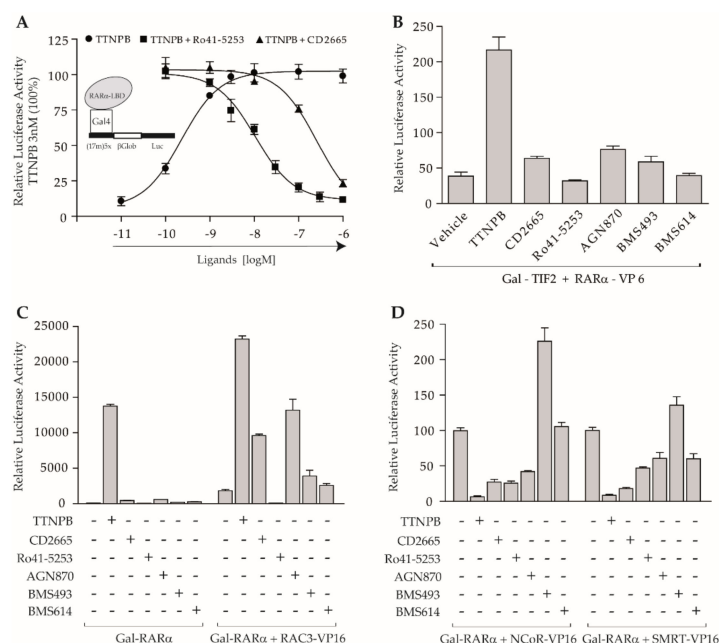
Figure 2. Co-regulator interactions define different classes of RAR \alpha antagonists. Transient transfections were performed in COS cells; (A) to assess antagonistic activities of CD2665 and Ro41-5253 cells were co-transfected with (17m)5x- \beta Glob-Luc and Gal-RAR \alpha . The reporter was activated by 3 nM TTNPB (100%) and increasing concentrations of CD2665 (closed triangles) or Ro41-5253 (closed squares) were added in a concentration range of 10^{-10} to 10^{-6} M, as indicated. To assess the agonistic activity of TTNPB, cells were incubated with increasing concentrations of TTNPB alone in a range of 10^{-11} to 10^{-6} M (closed circles); (B) mammalian two-hybrid assay with (17m)5x- \beta Glob-Luc and Gal-TIF2 as bait and VP16-RAR \alpha as prey was performed to assess the influence of indicated retinoids on interaction between RAR \alpha and TIF2; (C) mammalian two-hybrid assays with Gal-RAR \alpha and RAC3-VP16 (right panel) were performed to reveal the partial agonist activity of RAR \alpha antagonists. Gal-RAR \alpha used alone (left panel); (D) mammalian two-hybrid assays with (17m)5x- \beta Glob-Luc and VP16-RAR \alpha and Gal-NCoR (left panel) or Gal-SMRT (right panel) were performed to assess the influence of indicated retinoids on interaction between RAR \alpha and CoRs (100%, basal transcriptional activity). Compounds were used at 1 \mu M in all two-hybrid assays. Error bars, s.e.m.
