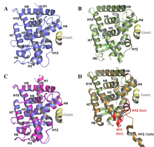
Figure 7. 3D crystal structure of RAR \beta and RXR \alpha LBDs in complex with LG754 and a coactivator peptides. (A) cartoon representation of RAR \beta LBD. Helices are numbered from H1 to H12, the latest being the activation helix that adopts the agonist conformation. The coactivator peptide (SCR1 NR2) bound to the surface formed by H3, H4, and H12 of RAR \beta is shown in yellow. The ligand LG754 is shown by stick representation; (B) cartoon representation of RXR \alpha LBD. The coactivator peptide (TIF2 NR2) bound to the protein is shown in yellow; (C) superposition of the two complexes of RAR \beta LBD bound to LG754 and coactivator peptide observed in the asymmetric unit; (D) superposition of our complex of RXR \alpha LBD bound to LG754 and coactivator peptide (same as in B) with the crystal structure of RXR \alpha LBD bound to LG754 in the context of the heterodimer RAR \alpha -RXR \alpha [69] (PDB code 3a9e). In the latest structure, the activation helix H12 adopts an antagonist position protruding outside the LBD, whereas, in the present structure (PDB code 6sti), helix H12 (shown in red) folds back on the LBD in the agonist position.
