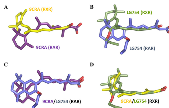
Figure 9. Conformation of the bound LG754 in RAR \beta and RXR \alpha . (A) superposition of 9CRA as seen in the LBP of RXR \alpha (PDB code 1fby) [70] and RAR \beta (PDB code 1xdk) [71]; (B) superposition of LG754 as seen in the LBP of RXR \alpha (PDB code 6sti) and RAR \beta (PDB code 6ssq); (C) superposition of LG754 and 9CRA as seen in the LBP of RAR \beta (PDB code 6ssq) and of 9CRA as seen in the LBP of RAR \beta (PDB code 1xdk) [71]; (D) superposition of LG754 as seen in the LBP of RXR \alpha (PDB code 6sti) and of 9CRA as seen in the LBP of RXR \alpha (PDB code 1fby) [70].
