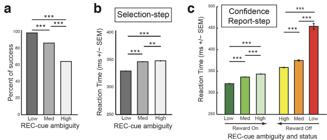
Figure 2. Impact of REC-cue ambiguity on behavioral confidence. (a) The rate of task success decreased significantly as the REC-cue ambiguity level increased ( \chi^2 -test, ***P < 0.001 ). (b) Reaction time (RT) increased significantly with the REC-cue ambiguity level during the Selection-step ( ***P < 0.001 ; **P < 0.01 for Bonferroni's post hoc test). (c) RTs during the Confidence-Report-step were significantly dependent on REC-cue ambiguity level, and were oppositely modulated according to “On”/“Off” reward status ( ***P < 0.001 for Bonferroni's post hoc test). All RT values in (b,c) are means \pm SEM. Note that as in Fig. 1c the level of ambiguity is displayed in an inverse manner for “On” and “Off” REC-cue status as indicated by arrows.
