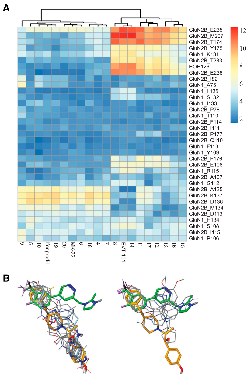
Fig. 4. In silico docking analysis of structurally-diverse GluN2B antagonists. (A) Protein-ligand fingerprints ("heat-maps") based on the EVT-101 protein cocystal structure and displaying computed amino acid-ligand distances. Amino acids are organized according to interaction distance (color code indicates minimal distance to ligands, in Å); numbers on the x-axis represent ligands listed in Table 2. Data show two distinct groups of ligands (see arborization on top) indicating at least two main modalities of binding. (B) Pose overlay for the two groups of compounds. Green: EVT-101; orange: ifenprodil. MK-22 depicted as overlapping with ifenprodil on the left in cyan.
