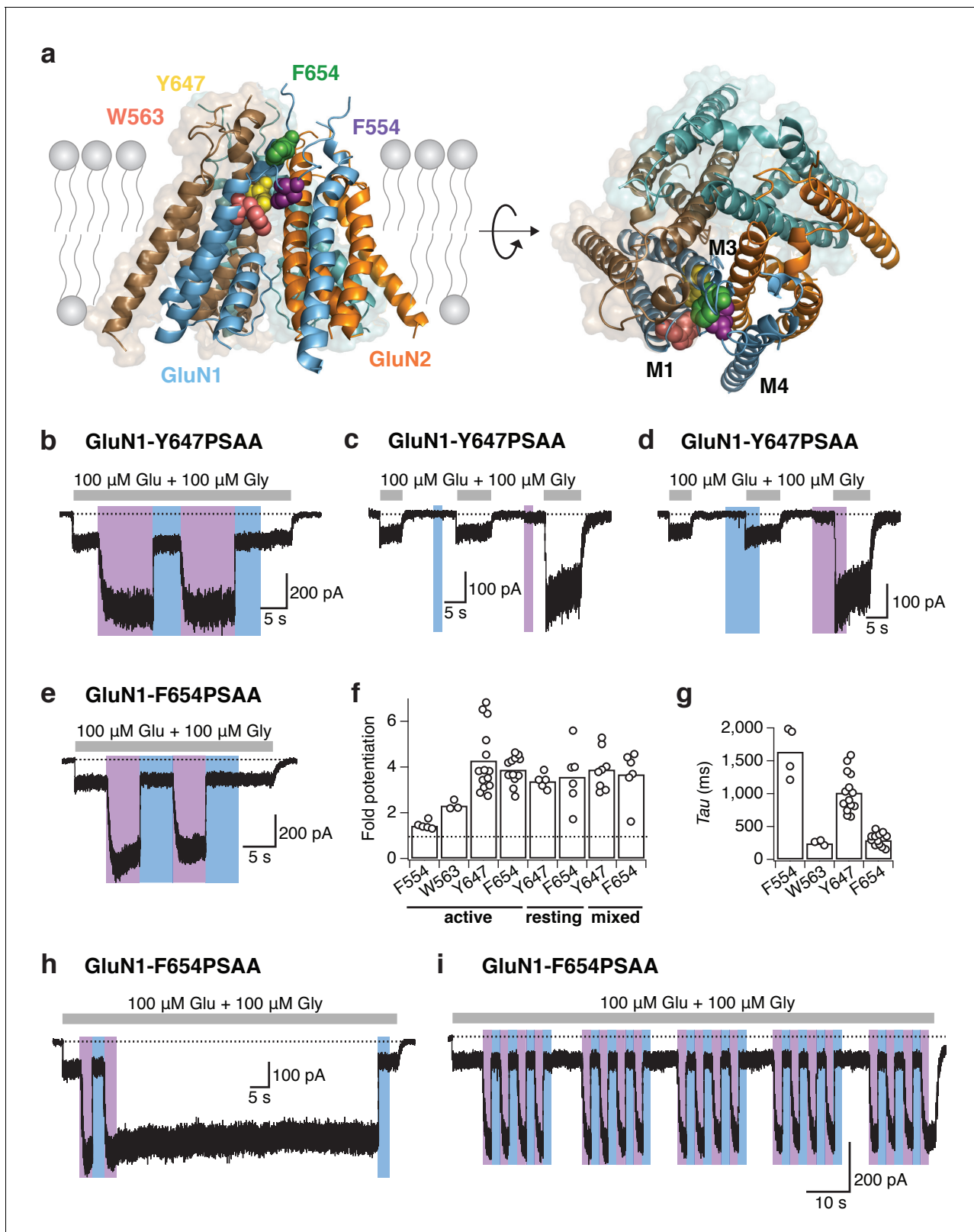
Figure 6. Reversible NMDAR photopotential with PSAA at various pore sites. (a) Structure of the GluN1/GluN2 TMD represented by a side (left panel) and top view (right panel). The four sites of the hydrophobic cluster, where PSAA was incorporated, are illustrated as spheres in different colors. (b) Example recording for GluN1-647PSAA/GluN2A mutants. UV illumination in the presence of the co-agonists resulted in a 3.4-fold potentiation of receptor activity. (c) Same cell as in b, with light applied in the resting state. Here, the UV-driven potentiation was 3.9-fold. (d) Same cell as in b, with Figure 6 continued on next page
