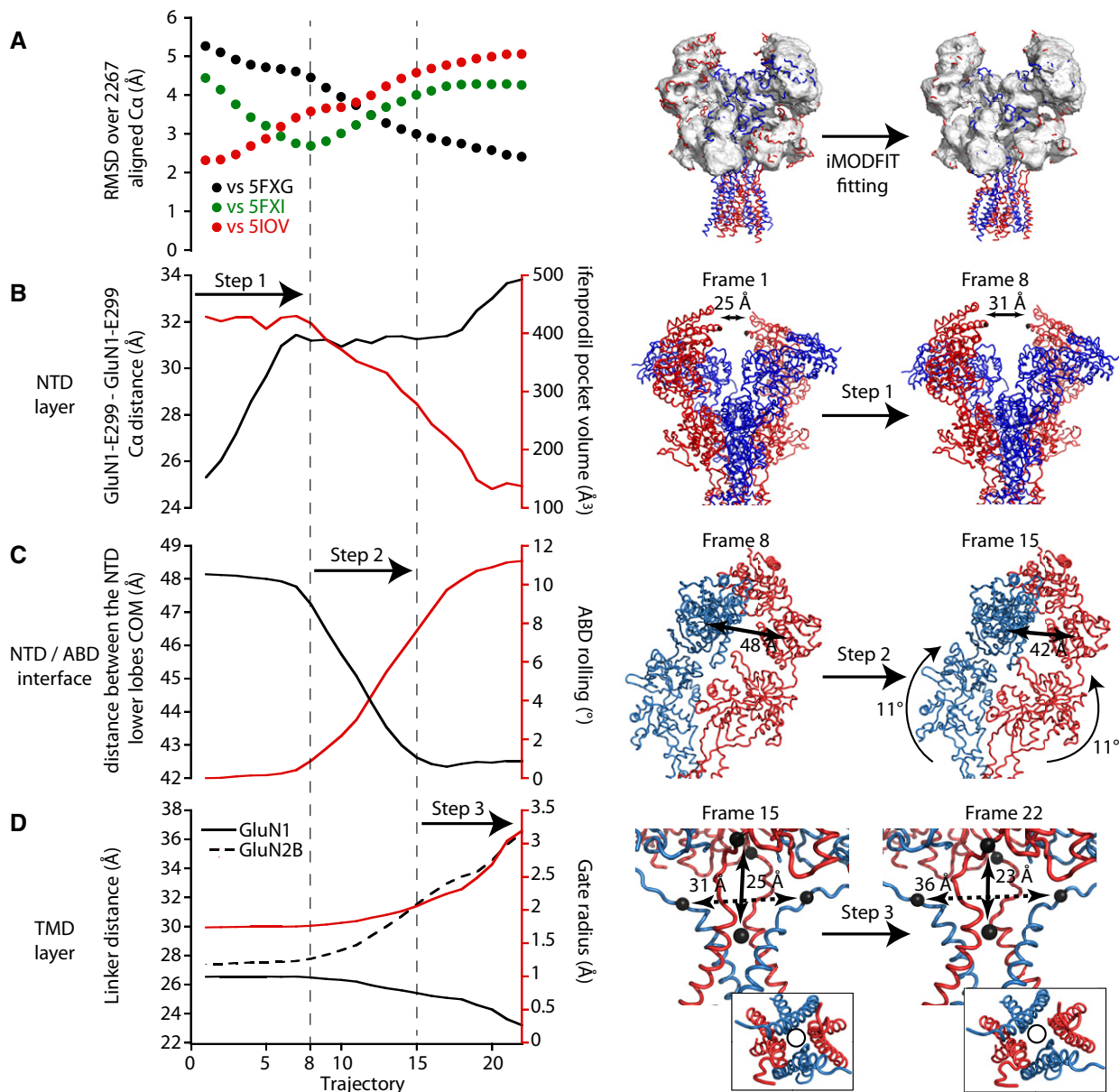
Figure 4. Rolling mediates inter-layer coupling and facilitates pore opening.
