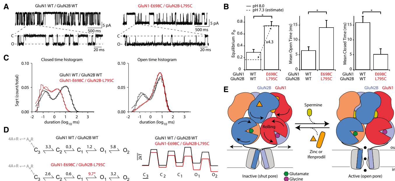
Figure 6. Influence of rolling on single-receptor gating kinetics.
