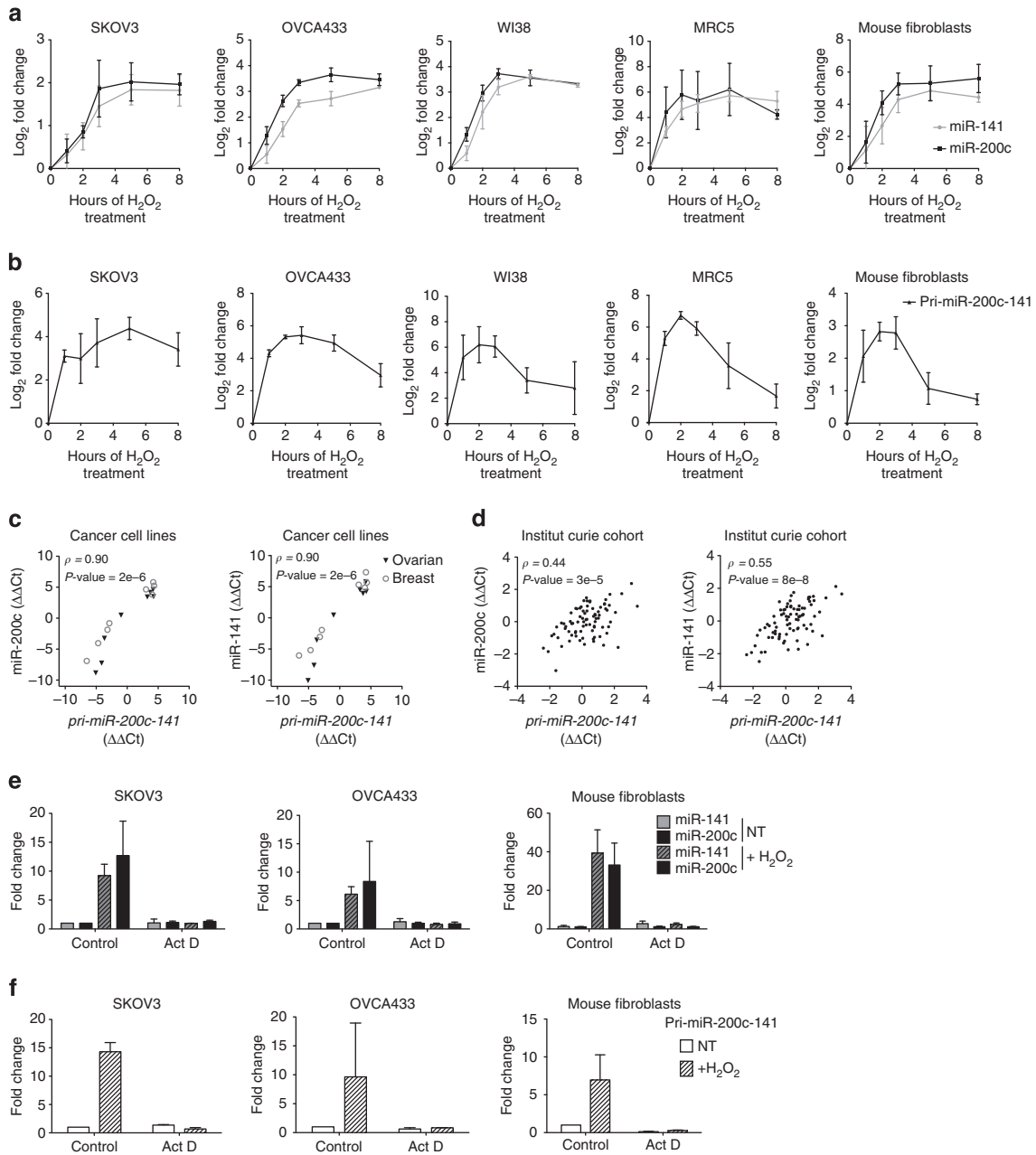
Figure 1 | Transcriptional regulation is crucial for miR-200c and miR-141 expression. (a,b) Kinetics of accumulation of miR-200c (black) and miR-141 (grey; a) and their corresponding primary transcript, pri-miR-200c-141 (b), following H 2 O 2 treatment in human ovarian cancer cell lines (SKOV3, OVCA433), human (WI38, MRC5) and mouse fibroblasts, as indicated. qRT-PCR data are means of fold changes (normalized to untreated and expressed as log 2 ) ± s.d. n = 3 independent experiments at least, except for OVCA433, n = 2 (in this case error bars indicate range of data). Kinetics of accumulation in eight other cell lines can be found in Supplementary Fig. 1. Sequences of the pri-miR-200c-141 F/R primers from mouse or human origins are given in Supplementary Table 2. (c,d) Scatter plots showing that levels of miR-200c (left) and miR-141 (right) are correlated with pri-miR-200c-141 primary transcript levels in ovarian (IGROV-1, OV90, OV2008, OVCAR3, OVCA433, RMG1, SHIN3, SKOV3) and breast (SKBr3, MDA-MB-468, MCF7, MDA-MB-231, MDA-MB-436, MDA-MB-453, BT549) cancer cell lines (c) and in HGSOC (d). qRT-PCR data are shown as normalized cycle threshold centred to the mean (ΔΔCt). Spearman correlation coefficients ρ (rho) and corresponding P-values are indicated on each graph. n = 3 independent experiments per cell line, except for OVCAR3 cells, n = 2. (e,f) Effect of the transcription inhibitor actinomycin D (Act D) on the levels of miR-141 (grey) or miR-200c (black) (e) and their corresponding primary transcript, pri-miR-200c-141 (f), under untreated conditions (NT) or following 3 h of H 2 O 2 treatment (+H 2 O 2 ). Cells were pretreated for 4 h with Act D or dimethylsulphoxide (control). qRT-PCR data are shown as fold change ± s.d. of treated compared with untreated cells. n ≥ 2 independent experiments per cell line.
