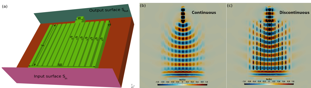
Fig. 1. (a): schematic view of the 3D photonic metalens. The structure consists of Si region (green part) on top of substrate made of SiO 2 (red part). The Si region is divided into three parts; the input port with width W = 3000 nm, the output port with width w = 300 nm, and in between we have several Si strips with length L and height h = 310 nm. The input mode is injected from the surface S_{in} (solution of the 2D modal problem) and the objective function is computed at the output surface S_{out} as the overlap between the obtained solution and the solution to the 2D modal problem at this surface. The widths of the strips are denoted by e_i, i \in \{0, 6\} . (b) and (c) represent the \Re e(H_y) and the \Re e(E_x) , of the optimized design, respectively.
