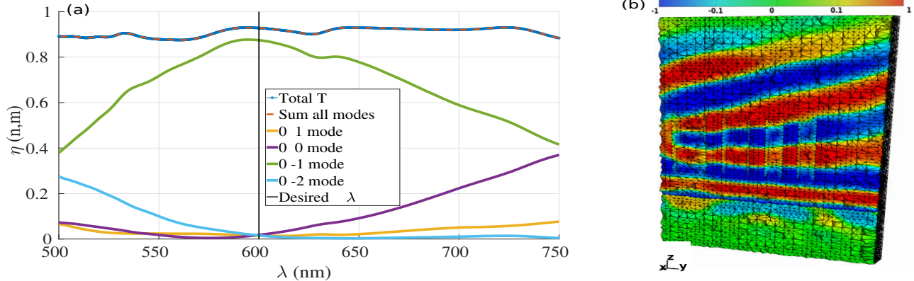
Figure 2: (a): Diffraction efficiency \eta(n, m) for the main modes as a function of the wavelength, the total transmission is shown in blue. (b); \Re(E_y) obtained from our DGTD solver [8] at \lambda = 600nm .
