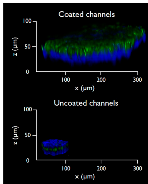
Figure 6. Three-dimensional analysis of 3D microtissues produced in gelatin-coated microchannels (top) and in control uncoated microchannels (bottom). The 3D reconstruction is the projection along z-axis of confocal z-sectioning images (z-slice thickness = 5.28 \mu\text{m} ). The depicted experiment was carried out in triplicate.
