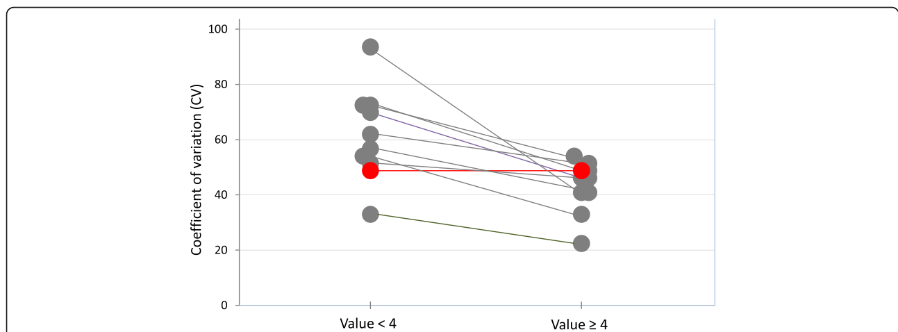
Fig. 2 Coefficient of variation (CV) values allowed the categorization of the perception of future and current risk in two classes based on a cut-off of 4 ( < 4 and \geq 4 ) that described the main trend for the different situations and different arboviral diseases. Generally (dots in grey color), the coefficients of variation (CV) values were higher for values lower than 4 (corrected CV = range values between 36.160 and 93.415, p < 0.001 ) than for values higher or equal to 4 (corrected CV = range values between 22.004 and 50.095, p < 0.001 ). Conversely, for the imported cases of dengue nation-wide (in red color), the variation coefficients were identical in both groups (corrected CV = 43.553 and 44.420, respectively, p = 0.995 ). See text for further details
