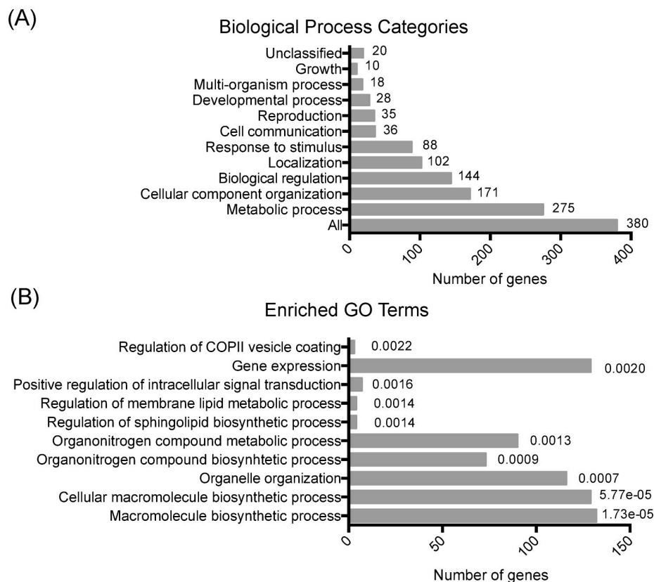
Fig 1. GO term enrichment for genes present in the QTLs genomic intervals. The GO classification (A) and enrichment analysis (B) for the 380 genes present in 26 QTLs identified by Cubillos et al. [20]. In panel A, the values represent the number of genes for each category. In panel B, the P values for each enrichment category are shown (Benjamini-Hochberg procedure).
