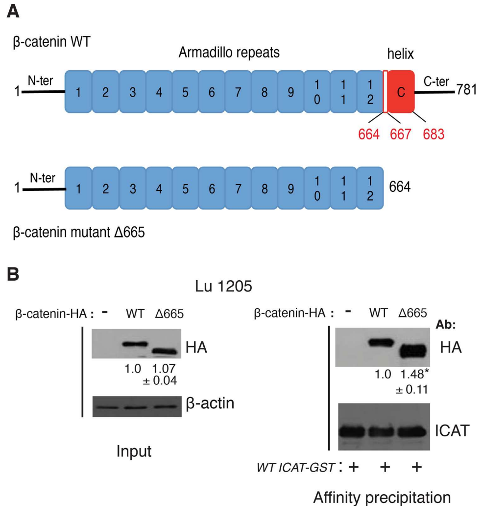
Fig 5. The lack of helix C in \beta -catenin does not prevent interaction with ICAT. A. Schematic representation of WT and mutant \Delta 665 HA-tagged \beta -catenin-NLS proteins. B. Total cell lysates from Lu1205 cells transfected with WT or mutant \beta -catenin \Delta 665 were analyzed by WB or affinity immunoprecipitated with WT ICAT-GST recombinant protein and blotted with anti-HA and anti-ICAT antibodies. Numbers represent mean \pm SD of normalized densitometry values from three independent experiments, * p < 0.05 .
