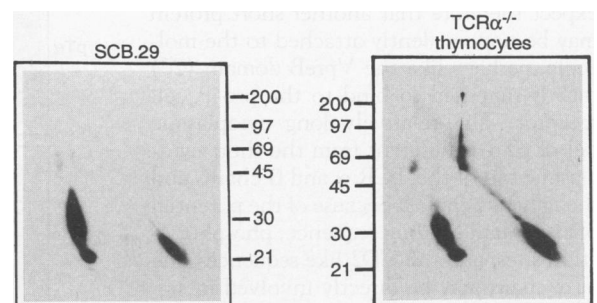
Fig. 2. Identification of the pT \alpha chain in TCR \alpha -/- thymocytes ( 4 \times 10^9 cells) and SCB.29 ( 2 \times 10^7 cells). Two-dimensional SDS-PAGE of immunoprecipitates with H57 (17). The pT \alpha chain is revealed by CP53 serum. The spot on the diagonal may represent nondisulfide-linked pT \alpha in the precipitate. Staining with mAb F23.1 was similar to that in Fig. 1. Methods were as in Fig. 1. Molecular sizes are indicated in kilodaltons.
