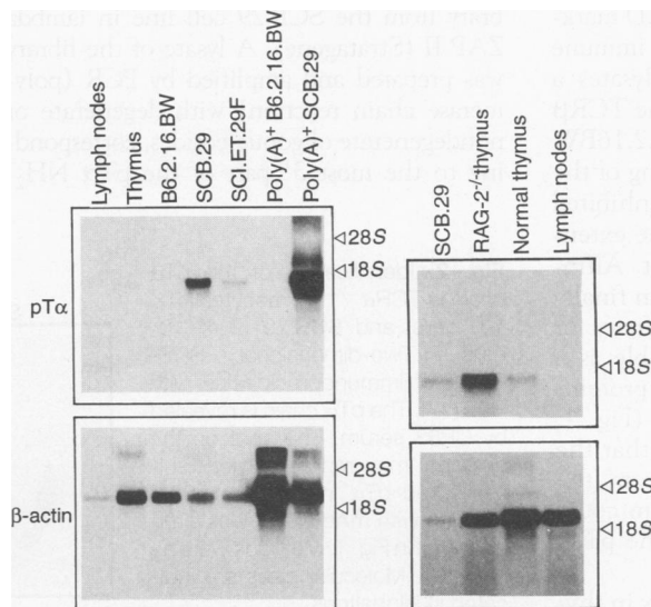
Fig. 4. pT \alpha mRNA expression in various cells and tissues. Total or poly(A) + RNA was isolated from cell lines and tissues and the RNA was separated on agarose gels. After transfer, the RNA was probed with a labeled cDNA specific for pT \alpha ; after the original probe was stripped from the filter, it was again hybridized with a labeled \beta -actin probe (41).
