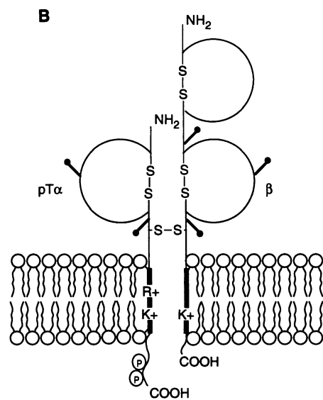
Fig. 3. (A) Predicted pT \alpha sequence. Amino acid sequence of the open reading frame of pT \alpha cDNA. The nucleotide sequence is available from the GenBank database, accession number U16958. Amino acid numbering is given at the left. Locations of the potential N-linked glycosylation sites (CHO), the predicted leader (peptide signal) and transmembrane (TM) sequences, and the potential protein kinase C phosphorylation sites (PKC) are shown. The sequences PPSRK (169) and PPTHR (176) are similar to the PPGHR motif found in CD2. The three cysteines in positions 31, 91, and 119 are marked (V). DNA sequence analysis was done with the GCG program (Genetics computer group, program manual for the GCG package, version 7, April 1991). Homology searches in the EMBL (release 33.0, March 1994), GenBank (release 83.0, February 1994) and SWISSPROT (release 28.0, February 1994) data banks were done with the FASTA (39) program. Sequence comparisons and alignments with immunoglobulin superfamily domains were done with the PILEUP (40) program. Single-letter abbreviations for the amino acid residues are: A, Ala; C, Cys; D, Asp; E, Glu; F, Phe; G, Gly; H, His; I, Ile; K, Lys; L, Leu; M, Met; N, Asn; P, Pro; Q, Gln; R, Arg; S, Ser; T, Thr; V, Val; W, Trp; and Y, Tyr. (B) The pT \alpha -TCR \beta complex. ●, Corresponds to the N-linked glycosylation sites. P, represents protein kinase C phosphorylation sites in the pT \alpha cytoplasmic tail. Two basic amino acids, arginine (R + ) and lysine (K + ), are located in the pT \alpha transmembrane region.
