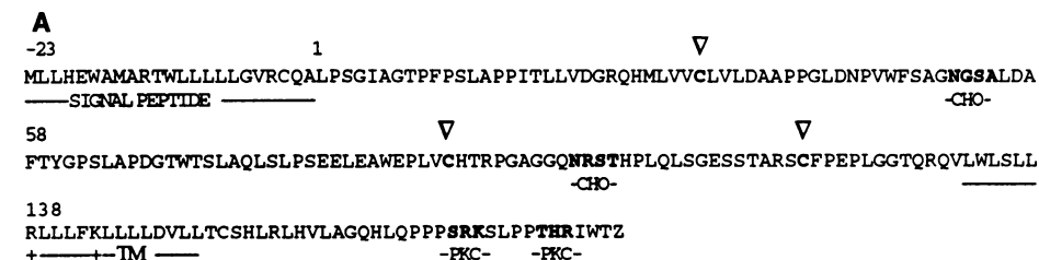
Fig. 3. (A) Predicted pT \alpha sequence. Amino acid sequence of the open reading frame of pT \alpha cDNA. The nucleotide sequence is available from the GenBank database, accession number U16958. Amino acid numbering is given at the left. Locations of the potential N-linked glycosylation sites (CHO), the predicted leader (peptide signal) and transmembrane (TM) sequences, and the potential protein kinase C phosphorylation sites (PKC) are shown. The sequences PPSRK (169) and PPTHR (176) are similar to the PPGHR motif found in CD2. The three cysteines in positions 31, 91, and 119 are marked (V). DNA sequence analysis was done with the GCG program (Genetics computer group, program manual for the GCG package, version 7, April 1991). Homology searches in the EMBL (release 33.0, March 1994), GenBank (release 83.0, February 1994) and SWISSPROT (release 28.0, February 1994) data banks were done with the FASTA (39) program. Sequence comparisons and alignments with immunoglobulin superfamily domains were done with the PILEUP (40) program. Single-letter abbreviations for the amino acid residues are: A, Ala; C, Cys; D, Asp; E, Glu; F, Phe; G, Gly; H, His; I, Ile; K, Lys; L, Leu; M, Met; N, Asn; P, Pro; Q, Gln; R, Arg; S, Ser; T, Thr; V, Val; W, Trp; and Y, Tyr. (B) The pT \alpha -TCR \beta complex. ●, Corresponds to the N-linked glycosylation sites. P, represents protein kinase C phosphorylation sites in the pT \alpha cytoplasmic tail. Two basic amino acids, arginine (R + ) and lysine (K + ), are located in the pT \alpha transmembrane region.
