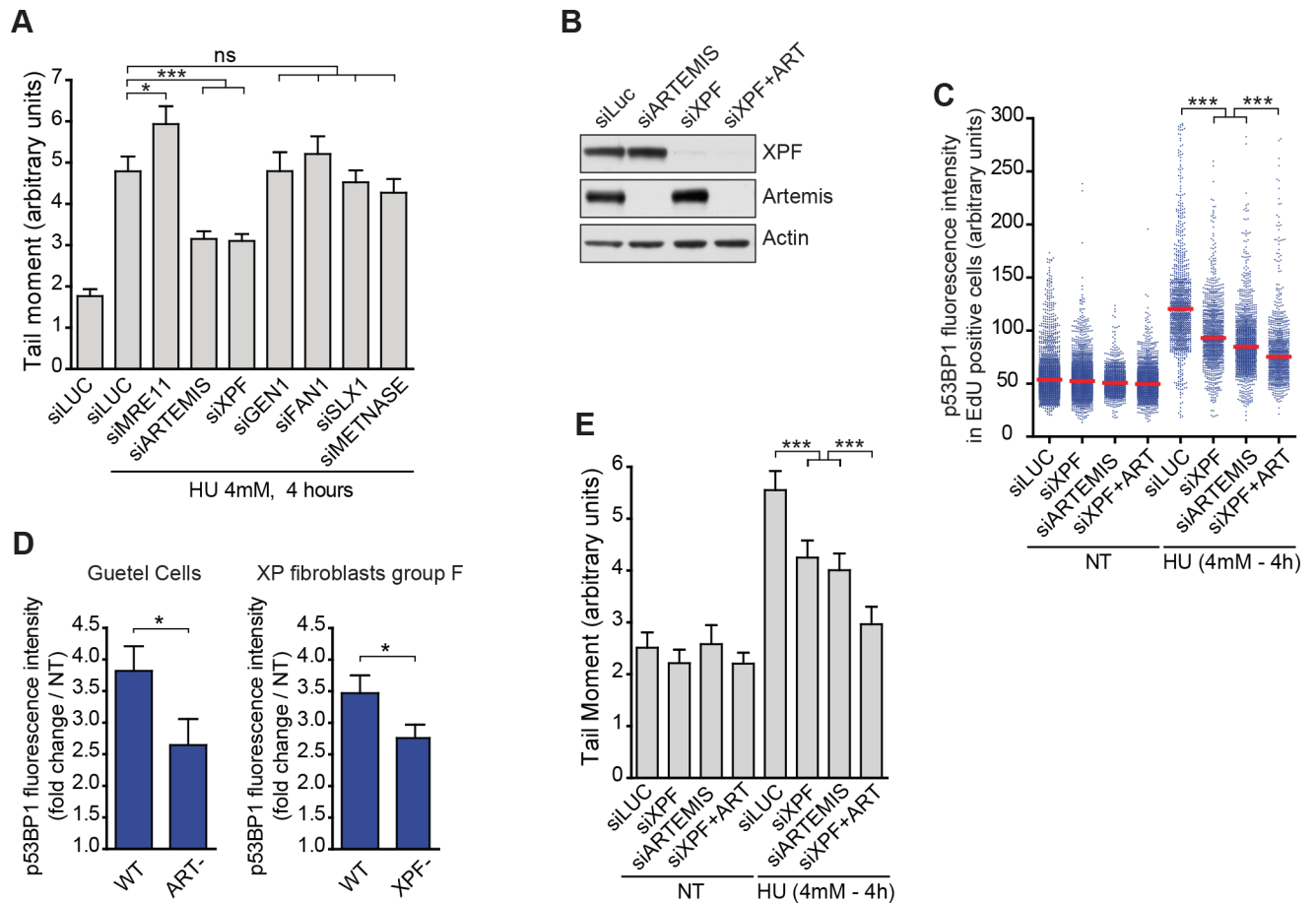
Fig 3. ARTEMIS and XPF are involved in RRFB. (A) Quantification by neutral comet assay of DSBs induced in response to treatment with 4 mM HU for 4 hours in control cells (siLUC) and in cells depleted of one of various endonucleases. The plot shows mean tail moment (% DNA in tail x tail length). Error bars represent SEMs. At least 150 comets were scored. * p < 0.05 , *** p < 0.0001 (Mann–Whitney test). (B) Western blots of whole cell extracts of RKO cells showing depletion of Artemis (siARTEMIS), XPF (siXPF) and both (siXPF + ARTEMIS). (C) Quantification of nuclear p53BP1 fluorescence intensity by QIBC in >1500 S-phase RKO cells depleted of XPF and/or ARTEMIS and either untreated (NT) or treated with 4 mM of HU for 4 hours, as indicated. *** p < 0.0001 (Mann–Whitney test). (D) Quantification of nuclear p53BP1 fluorescence intensity by QIBC in Artemis-deficient RS-SCID patient cells (Guetel cells) and in XPF-deficient XP patient cells (XP fibroblasts group F) compared to WT primary fibroblasts. Mean fold change compared to untreated cells is shown. Error bars represent standard deviations from 3 independent experiments. * p < 0.05 (Student's T test). (E) Quantification by neutral comet assay of DSBs in untreated RKO cells (NT) and in cells treated with 4 mM HU for 4 hours after depletion of XPF and/or ARTEMIS, as indicated. The plot shows mean tail moment (% DNA in tail x tail length). Error bars represent SEMs. At least 150 comets were scored. *** p < 0.0001 (Mann–Whitney test).
