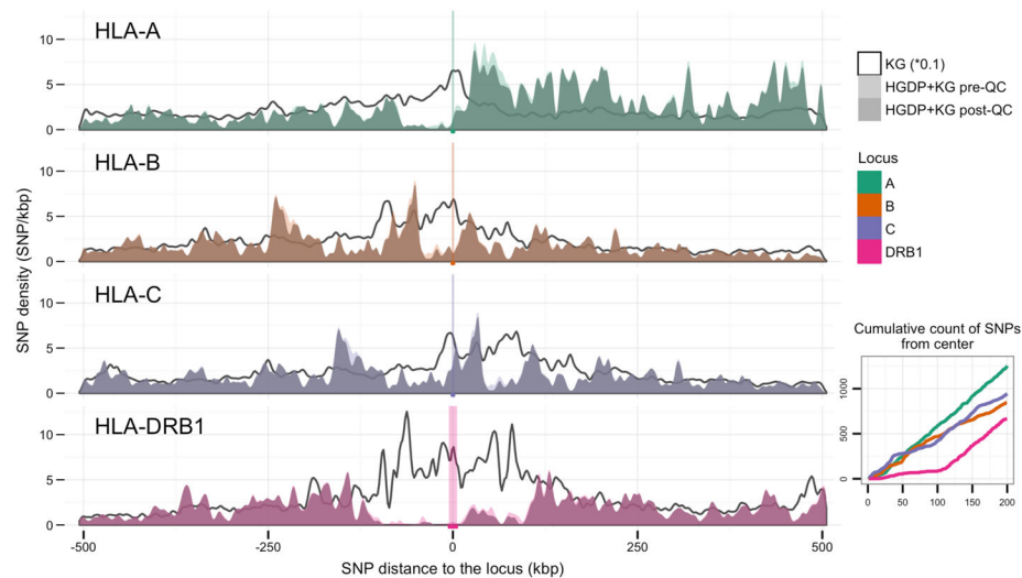
Figure 6. SNP Proximity and Density for the HLA-A, -B, -C and DRB1 Loci
