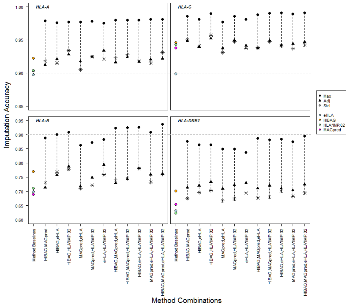
Figure 5. Maximum, Adjudicated and Standardized Imputation Accuracies in Method Combinations
