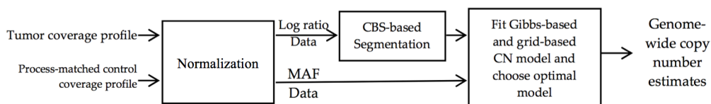
Fig 2. Copy number detection overview. Aligned DNA sequences of the tumor specimen are normalized against a process-matched normal, producing log-ratio and minor allele frequency (MAF) data. Next, whole-genome segmentation is performed using a circular binary segmentation (CBS) algorithm on the log-ratio data. Then, a Gibbs sampler fitted copy number model and a grid-based model are fit to the segmented log-ratio and MAF data, producing genome-wide copy number estimates. Finally, the degree of fit of candidate models returned by Gibbs sampling and grid sampling are compared and the optimal model is selected by an automated heuristic.
