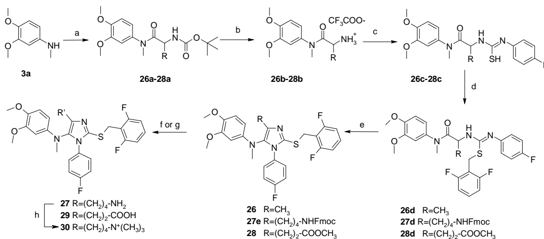
Scheme 12. Synthetic route to 26-30 .
