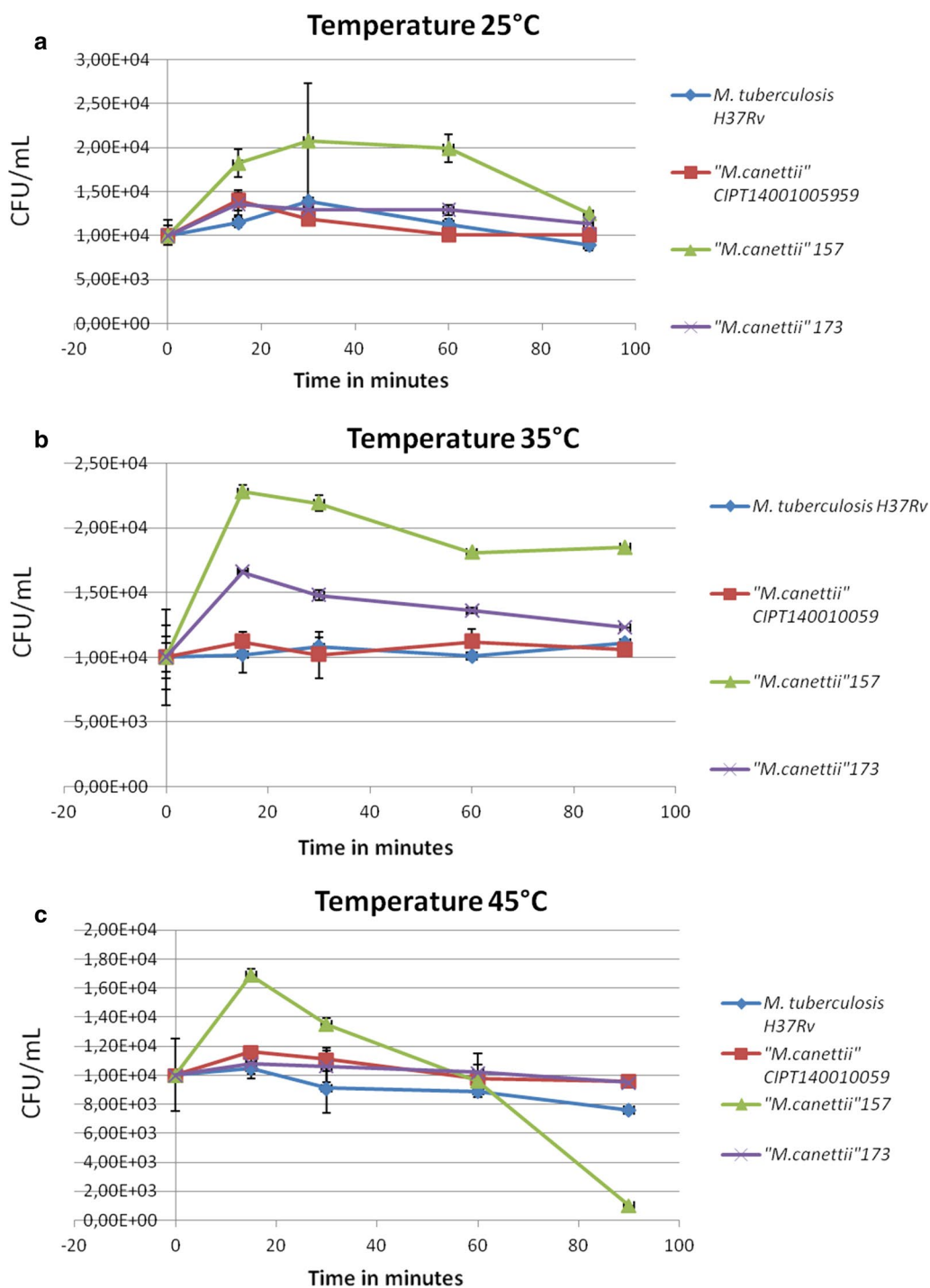
Fig. 1 Survival curves for M. tuberculosis H37Rv, " M. canettii " CIPT140010059, " M. canettii " 157 " M. canettii " 173 a 25 °C, b 35 °C, c 45 °C
