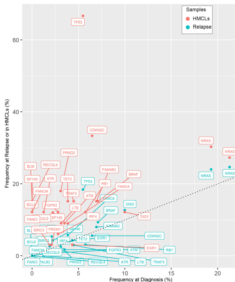
Fig. 2 Comparison of the gene mutation/deletion frequency in human myeloma cell lines with multiple myeloma patients at diagnosis and relapse. The frequency of mutation/deletion at diagnosis (x-axis) was plotted against that at relapse (y-axis, blue). HMCL hit frequencies are represented in red dots. The dashed line represents the theoretical identical ratio between diagnosis and relapse
