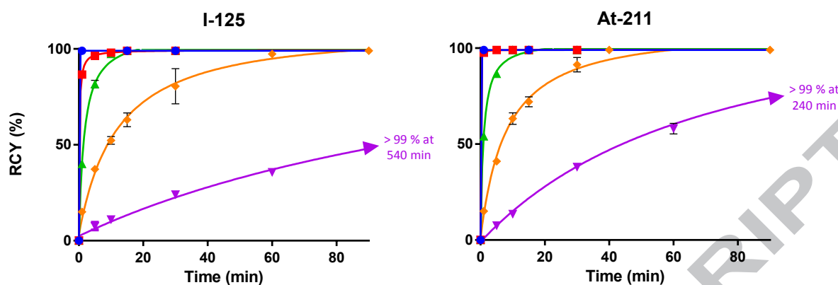
Figure 3. Kinetics of bioorthogonal conjugation between clickable peptides and radiohalogenated prosthetic groups ( n = 3 ): CuAAC (■); DIBAC/ N_3 -SPAAC (◆); BCN/ N_3 -SPAAC (▼); BCN/Tz-IEDDA (▲); TCO/Tz-IEDDA (●). RCYs based on the HPLC analysis of the crude product.
