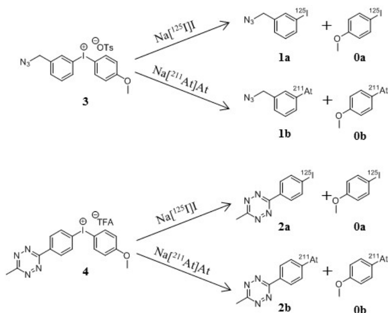
Scheme 3. Radioiodination and astatination of aryliodonium precursors 3 and 4 .
