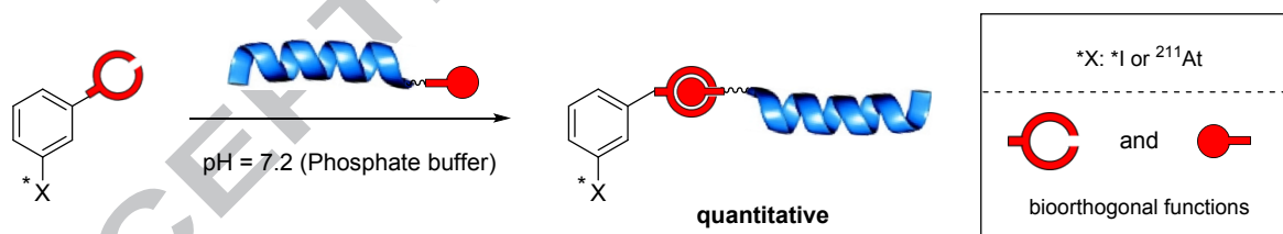
Figure 1. Bioconjugation strategies to form radiohalogenated proteins.
