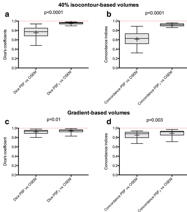
Fig. 5 Impact of the EARL harmonization strategy on Dice and concordance indices between MATVs extracted from OSEM images and PSF images (observer 1). The PSF 7 images were filtered to meet EARL requirements while PSF images were optimised for diagnostic potential. Data are shown as Tukey boxplots (lines displaying the median, 25th, and 75th percentiles; crosses represents the mean values). Dice coefficients and concordance indices are shown for both the isocontour-based method ( a , b ) and gradient-based method ( c , d ). ns not significant
