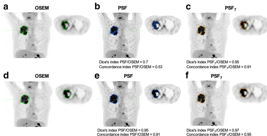
Fig. 6 Representative images of isocontour- and gradient-based automatic contouring of PSF images optimised for diagnostic and EARL-compliant purposes. Maximum intensity projections and transverse slices at the level of a necrotic tumour in the right upper lobe of the lung are shown for OSEM, unfiltered PSF images, and PSF images filtered to meet EARL requirements (PSF 7 ). Dice and concordance indices are given for each contouring method, using the MATV extracted from the OSEM images as a reference standard
