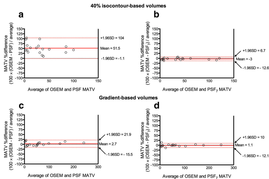
Fig. 4 Comparison of MATVs from PSF images optimised for diagnostic potential and EARL-compliant PSF 7 images (observer 1). Relationships between MATVs extracted from OSEM reconstructions and PSF or PSF 7 reconstructions, for the 40% isocontour-based methods ( a , b ) and gradient-based methods ( c , d ), assessed using Bland–Altman plots
