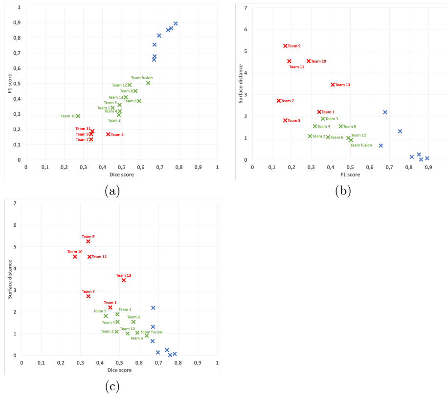
Figure 2: Graphical results illustration of automatic clustering of average results for each team and expert into three groups (scatter plots of pairs of two evaluation parameters: (a): Dice and F_1 scores, (b): surface distance and F_1 scores, (c): surface distance and Dice scores). Legend: blue crosses: group 1 (always containing only the seven experts even though the clustering is automatic), green crosses: group 2 (best performing algorithms), red crosses: group 3 (lower “quality” algorithms). Team numbers associated with each point on the graph are indicated as labels. Team fusion indicates a composite segmentation result further discussed in Section 2.5.
