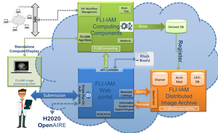
Figure 7: FLI-IAM architecture
