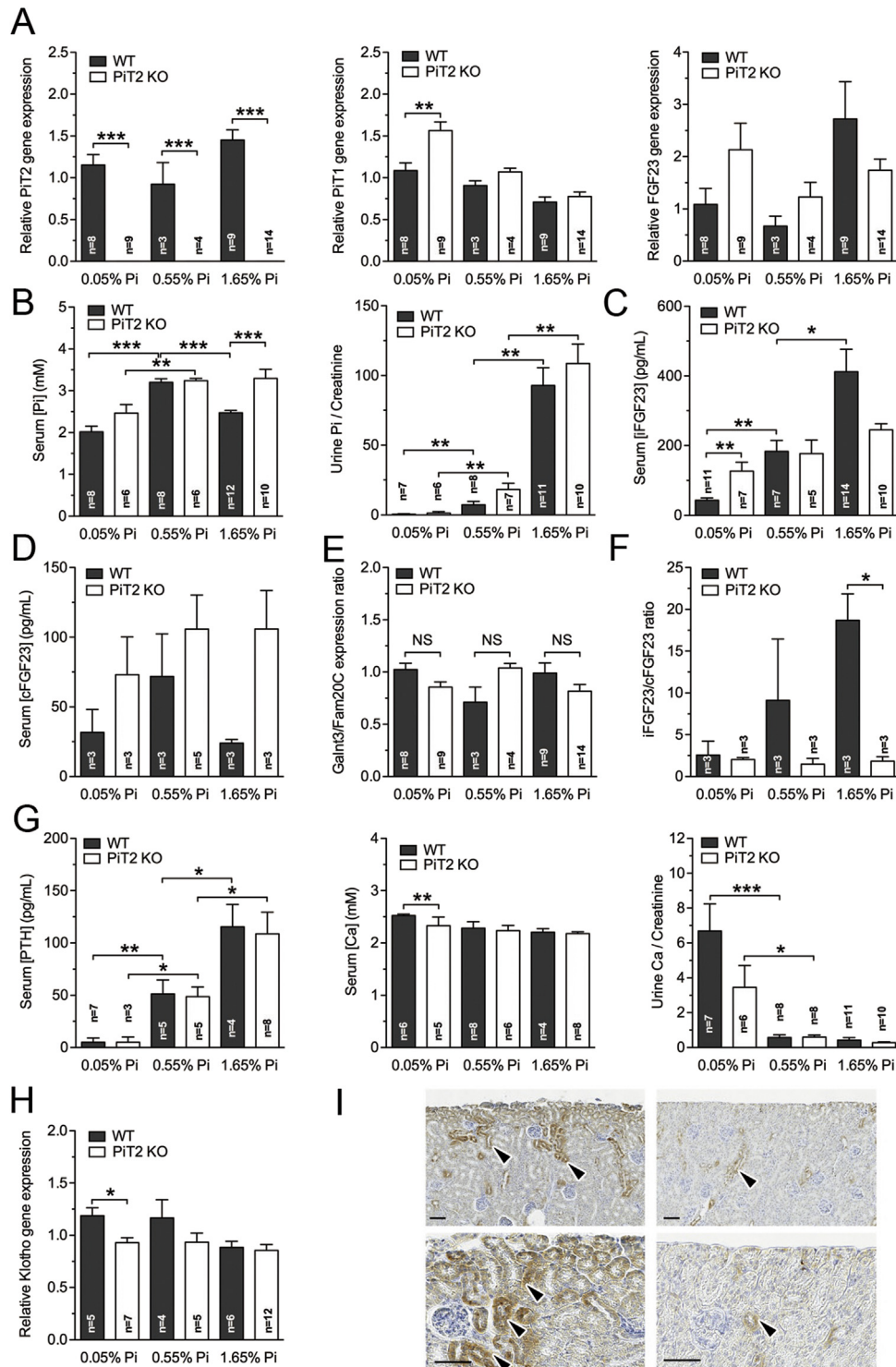
Figure 1: Deletion of Pit2 in vivo leads to inappropriate serum Fgf23 levels in low-Pi condition. (A) RT-qPCR analysis of Pit2 , Pit1 and Fgf23 mRNA levels in flushed tibiae isolated from WT or Pit2 KO mice fed with low (0.05%), normal (0.55%) and high (1.65%) Pi diets for one week. Pnn and Gusb genes were used as internal controls. (B) Serum and urine Pi values from WT or Pit2 KO mice fed with low (0.05%), normal (0.55%), and high (1.65%) Pi diets for one week. (C-D) Serum intact Fgf23 (iFgf23) (C) and C-terminal Fgf23 (cFgf23) (D) levels (ELISA) from WT or Pit2 KO mice fed with low (0.05%), normal (0.55%) and high (1.65%) Pi diets for one week. (E-F) Gaint3/Fam20C mRNA ratios as determined by RT-qPCR analysis (E) and iFgf23/cFgf23 ratios (F) from flushed tibiae from WT or Pit2 KO mice fed with low (0.05%), normal (0.55%) and high (1.65%) Pi diets for one week. Pnn and Gusb genes were used as internal controls. (G) Serum PTH levels (Left) and serum and urine Ca values (Center and Right) from WT or Pit2 KO mice fed with low (0.05%), normal (0.55%) and high (1.65%) Pi diets for one week. (H) RT-qPCR analysis of \alpha Klotho mRNA levels in kidneys isolated from WT or Pit2 KO mice fed with low (0.05%), normal (0.55%) and high (1.65%) Pi diets for one week. Pnn and Gusb genes were used as internal controls. (I) Immunohistochemistry for \alpha Klotho of kidney sections from WT or Pit2 KO mice fed with low (0.05%) Pi diet for one week. Black arrowheads: \alpha Klotho-positive staining. Top, low magnification; Bottom, high magnification, scale bar, 50 \mu m. Data are means \pm S.E.M. * p < 0.05, ** p < 0.01, *** p < 0.001, NS: not significant.
