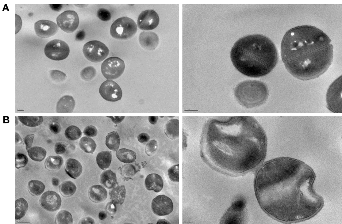
Figure 4 Transmission electron microscope images of MSSA ATCC strain untreated control (A) and treated with 3.2 mg/mL (32x MIC) of ML-LNCs (B) for 1 hour. Scale bars: (A) left: 0.2 μm, right: 0.2 μm; (B) left: 0.5 μm, right: 100 nm.
