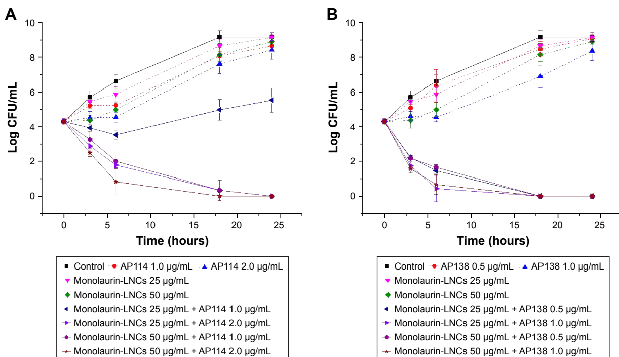
Figure 7 Time-kill curves of ML-LNCs and plectasin derivatives API 14 (A) and API 38 (B) used alone and in combination against MSSA ATCC strain.
