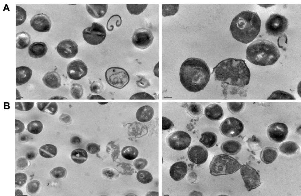
Figure 8 Transmission electron microscope images of MSSA ATCC strain treated with containing 1.6 mg/mL of ML-LNCs and plectasin derivative: 64 \mu\text{g/mL} of API 14 (A) or 32 \mu\text{g/mL} of API 38 for 1 hour. Scale bars: (A) left: 0.2 \mu\text{m} , right: 0.2 \mu\text{m} ; (B) left: 0.5 \mu\text{m} , right: 0.2 \mu\text{m} .
