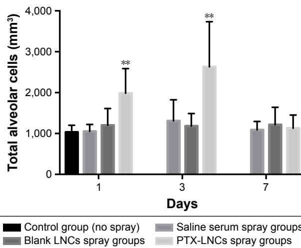
Figure 5 Mean ± SD of total alveolar cells for the control group (no spray), the saline serum spray group, the blank LNCs spray group and the PTX-LNCs spray group at days 1, 3 and 7 (n=6). Notes: Results indicate an increase in the total alveolar cells on the PTX-LNCs spray group only at days 1 and 3. At day 7, no difference is observed. ** p <0.01 versus the control group. Abbreviations: LNCs, lipid nanocapsule; PTX, paclitaxel; PTX-LNCs, PTX-loaded LNCs.
