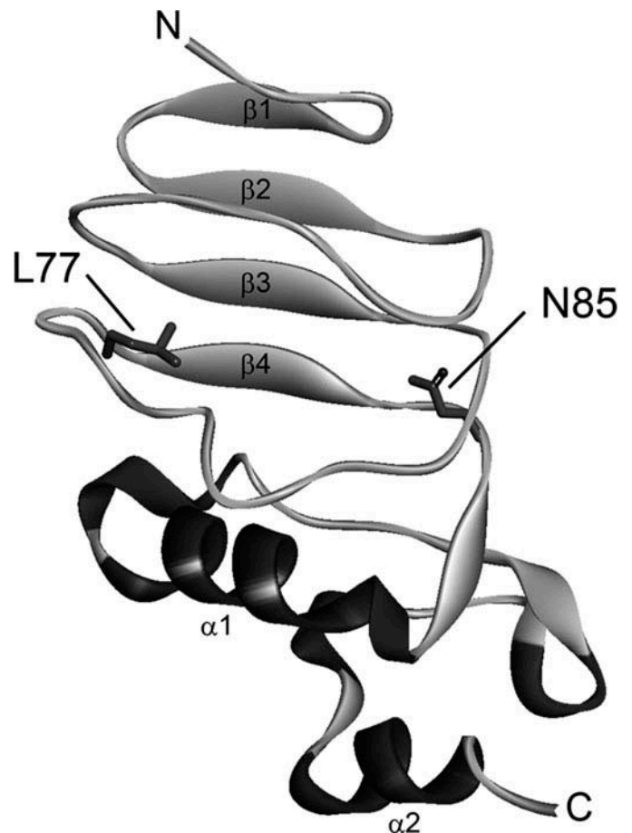
Figure 2. Crystal structure of GPIIb \beta Eabc, a GPIIb \beta /GPIIX ectodomain chimera. The structure of a chimera of GPIIb \beta and GPIIX ectodomains named GPIIb \beta Eabc (Protein Data Bank code 3REZ) in which three non-contiguous sequences that may constitute the putative convex surface of the GPIIb \beta ectodomain are replaced by their GPIIX counterparts [4] was used to visualize the position of the conserved residues Leu 77 and Asn 87. Ribbon diagram of the GPIIb \beta Eabc structure (PDB code 3REZ), with Leu residue 77 (L77) and Asn residue 85 (N85) shown as sticks.
