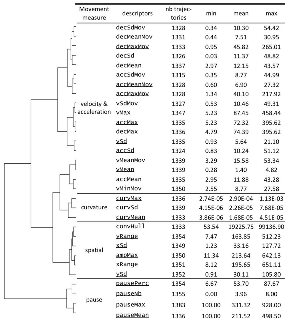
FIGURE 2 | Calculated descriptors of the trajectories. Data from a hierarchical clustering, using the Ward minimum variance method of the descriptors, is presented as a dendrogram to the left of the descriptors. Descriptors selected to be representative for each group of movement measures, based on their degree of dissimilarity, are underlined.
