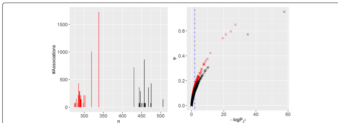
Fig. 3 \phi vs. -\log P_{\chi^2} across all the 8637 drug-gene associations from GDSC. (Left) Number of drug-gene associations for each number of tested cell lines (n). Two distinctive groups of drugs emerge: those tested on around 300 cell lines (red bars) and those tested around 450 cell lines (black bars). (Right) \phi versus -\log P_{\chi^2} across the drug-gene associations (same colour code). The Spearman and Pearson correlations between both metrics are 0.99 and 0.82, respectively. The vertical blue line marks the significance cutoff for the chi-squared test. The plot shows that all markers with an \phi of 0.15 or more are too discriminative to have arisen by chance (above an \phi of 0.12 if we restrict to the markers evaluated with more data shown as black crosses)
