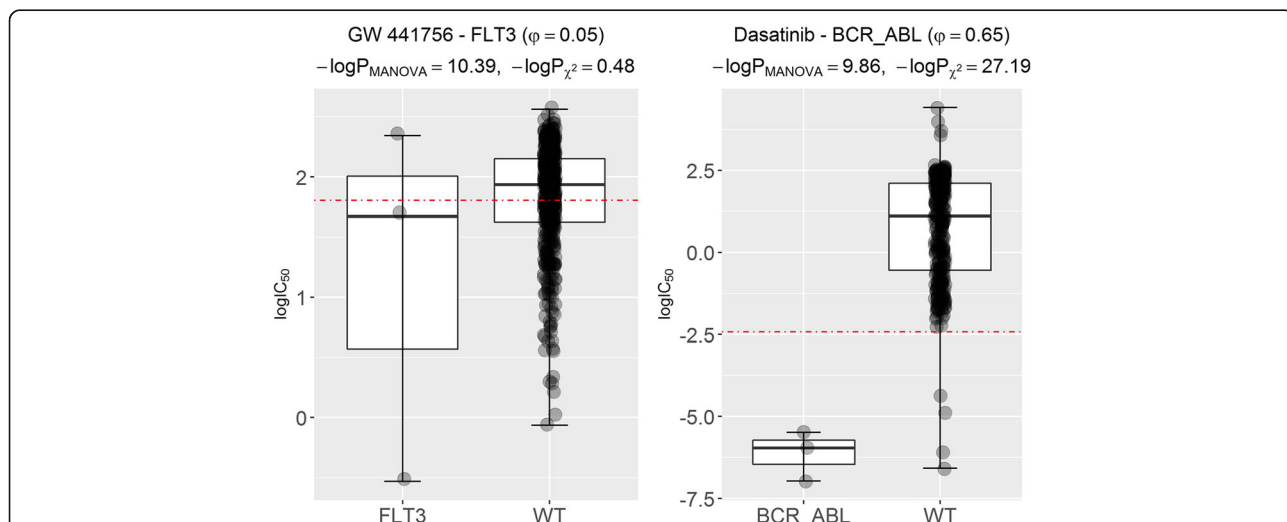
Fig. 4 Potential false-positive marker of the MANOVA test incorrectly rejected by the chi-squared test. (Left) The scatter plot for the drug-gene association (GW441756-FLT3) with the largest -\log P_{MANOVA} among those not significant according to the chi-squared test. Hence, mutated-FLT3 is a marker of sensitivity to the experimental drug GW441756 according to the MANOVA test, but not according to the chi-squared test. In the plotted training set, this marker offers practically no discriminative power as further evidenced by a \phi of just 0.05 and similar drug response ( \log C_{50} ) distributions of mutated and WT cell lines. However, this marker provides an MCC of 0.10 on the test and hence this is a false negative of the chi-squared test. (Right) Conversely, to assess the consistency of the MANOVA test, we searched for the drug-gene association with largest -\log P_{\chi^2} among those with a similar -\log P_{MANOVA} to that of GW441756-FLT3, which is Dasatinib-BCR_ABL. Whereas the p -value for Dasatinib-BCR_ABL is of the same magnitude as that for GW441756-FLT3 using the MANOVA test ( P_{MANOVA} \sim 10^{-10} ), the p -values for the same associations using the chi-squared test differ is almost 27 orders of magnitude. Thus, unlike the chi-squared test, the MANOVA test is unable to detect the extreme difference in discriminative power offered by these two drug-gene associations. Indeed, the BCR_ABL translocation is a highly discriminative marker of Dasatinib sensitivity ( \phi = 0.65 ), as also evidenced by the barely overlapping drug response distributions from each set of cell lines. This is confirmed in the test set, where the Dasatinib-BCR_ABL marker obtains an MCC of 0.21
