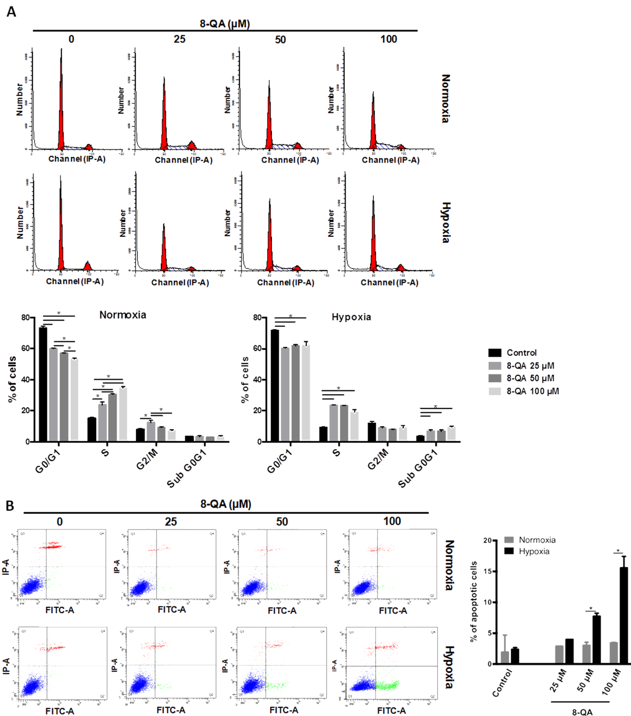
Figure 3: Cell cycle and apoptosis analyses on HEMC-SS cells treated by 8-QA. Cell cycle distribution (A) and Annexin V test (B) on HEMC-SS cells treated in normoxic (21% \text{O}_2 ) or hypoxic ( \text{N}_2 , \text{O}_2 < 0.3\% ) conditions by derivative 8-QA at 25 \mu\text{M} , 50 \mu\text{M} and 100 \mu\text{M} for 24 hours. (A) In normoxia, 8-QA treatment led to an increase in S-phase associated with a decrease in G2/M phase. In hypoxia, 8-QA treatment led to a high accumulation of cells in S-phase associated with an increase in SubG0/G1 phase. Data are represented as mean \pm SD. 8-QA treatments and controls were compared using two-way ANOVA analysis followed by Tukey's post-hoc multiple comparisons test. (B) Increase of Annexin V positive cells was observed after 8-QA treatment in hypoxia from 50 \mu\text{M} . Data are represented as mean \pm SD. Treatments in normoxic and hypoxic conditions were compared using a two-way ANOVA analysis followed by Bonferroni's post-hoc comparisons test.
