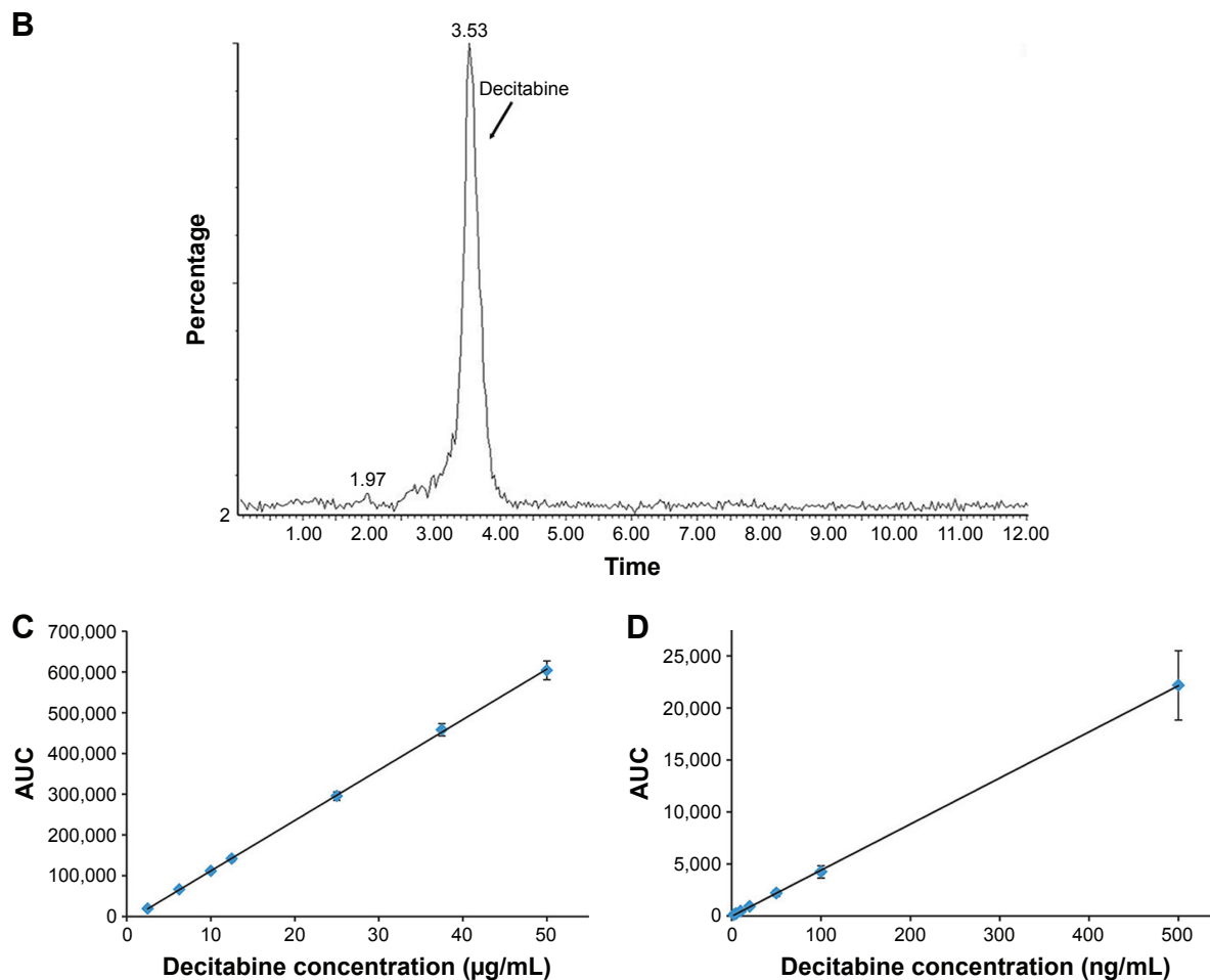
Figure S1 Chromatograms of a 40 µg/mL decitabine solution analyzed by the UPLC-UV method ( A ), a 20 ng/mL decitabine solution analyzed by the LC-MS/MS method ( B ), and mean calibration curves of the UPLC-UV method ( C ) and LC-MS/MS method ( D ).
