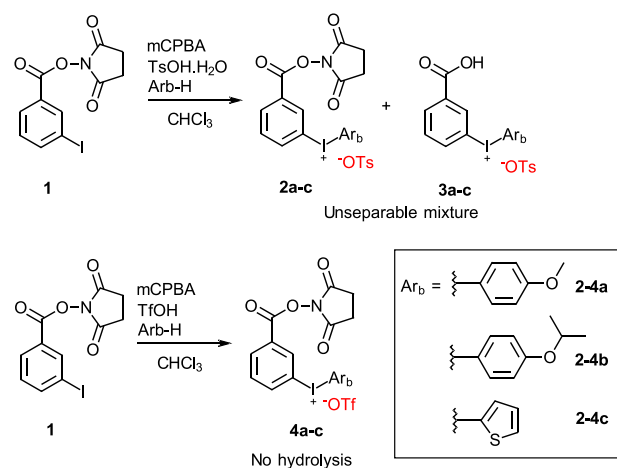
Scheme 2. Bifunctional arylidonium salts preparation
