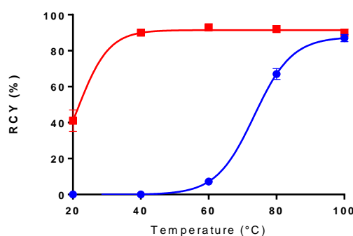
Figure 1. Influence of the temperature on the RCY of formation of [ 125 I]-SIB from 4c (●) and [ 211 At]-SAB from 4a (■) after 30 min in CH 3 CN determined by radio-HPLC analysis of the crude product (n ≥ 2).
