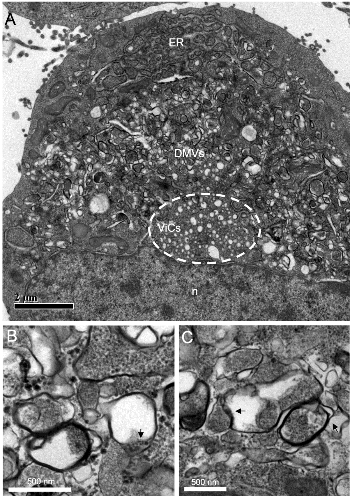
Fig.1. Membrane rearrangements encountered in HCV-infected cells.
