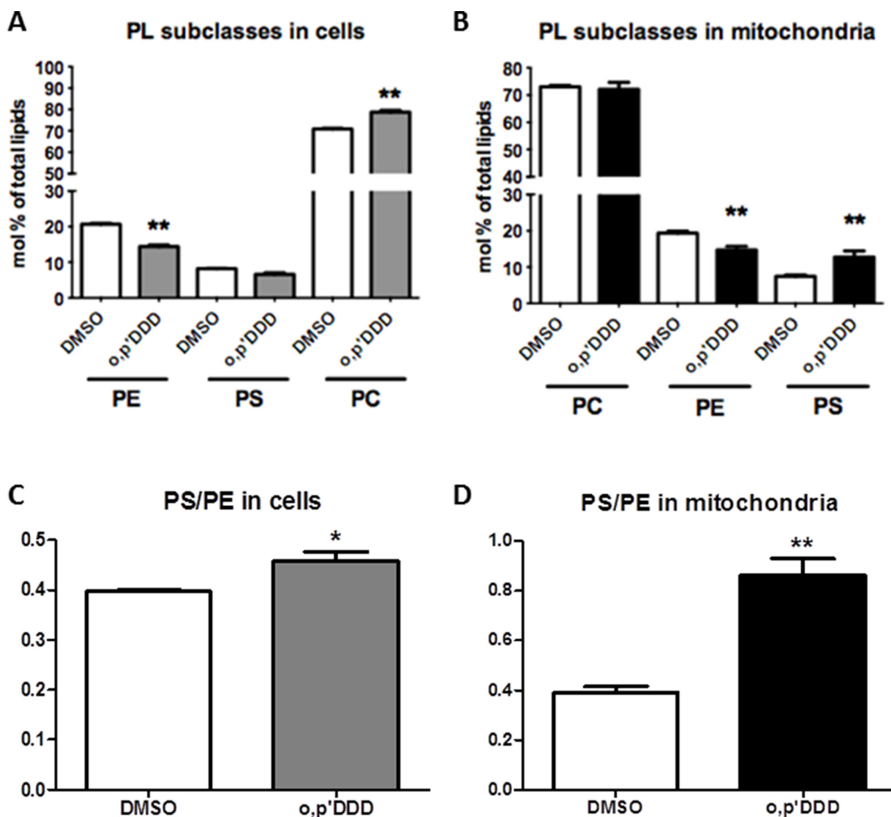
Figure 3: Lipidomic analyses of H295R cells and the corresponding mitochondrial fractions isolated as described in Material and Methods Section. H295R cells were treated with 50 \mu M for 48 h. PC: phosphatidylcholine, PE: phosphatidylethanolamine, PS: phosphatidylserine. (A) and (B) Levels of PC, PE and PS in H295R whole cells and isolated mitochondria expressed as molar percentage of total lipids. ( n = 6). (C) and (D) Molar ratio of PS/PE in H295R cells and isolated mitochondria. Results are means \pm SEM of 6 different experiments. * P < 0.05, ** P < 0.01 and *** P < 0.001, Mann-Whitney U -tests. Mitotane increases PS/PE ratio.
