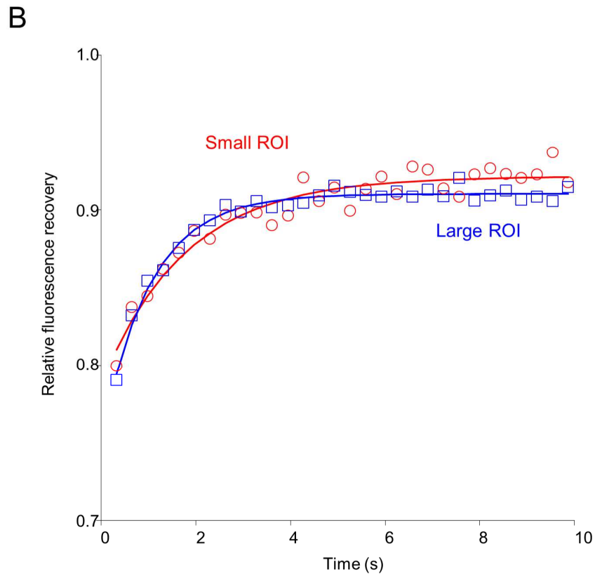
Figure S3. FRAP analysis of stathmin in the presence of MT. (A) left: enlarged view of stathmin fluorescence and MTs (inset); right: stathmin fluorescence recovery at exponentially increasing time points on the region containing MTs (ROI: 4 \mu\text{m} radius). (B) Mean data for small (2 \mu\text{m} radius) and large (4 \mu\text{m} radius) bleached ROIs, normalized to the first prebleach value, showing fluorescence recovery of stathmin. Recovery curves were fitted using a single exponential equation ( F(t) = F_{\infty} - C_{\text{eq}} \cdot \exp^{-k \cdot t} ) with no foreknowledge of either the geometry of the bleaching or the process of fluorescence recovery. Fits of data (small ROI, in red; large ROI, in blue) to the binding-dominant model give comparable fractions of fluorescence at equilibrium due to binding (small ROI: C_{\text{eq}} = 0.13 \pm 0.01 ; large ROI: C_{\text{eq}} = 0.15 \pm 0.02 ), dissociation rate constants (small ROI: k = 0.57 \pm 0.07 \text{ s}^{-1} ; large ROI: k = 0.49 \pm 0.06 \text{ s}^{-1} ), and fluorescence intensities (small ROI: F_{\infty} = 0.92 \pm 0.01 ; large ROI: F_{\infty} = 0.91 \pm 0.01 ). These features indicate that diffusion is not significantly limiting during recovery of stathmin in the presence of MT; recovery is instead dominated by binding interactions.
