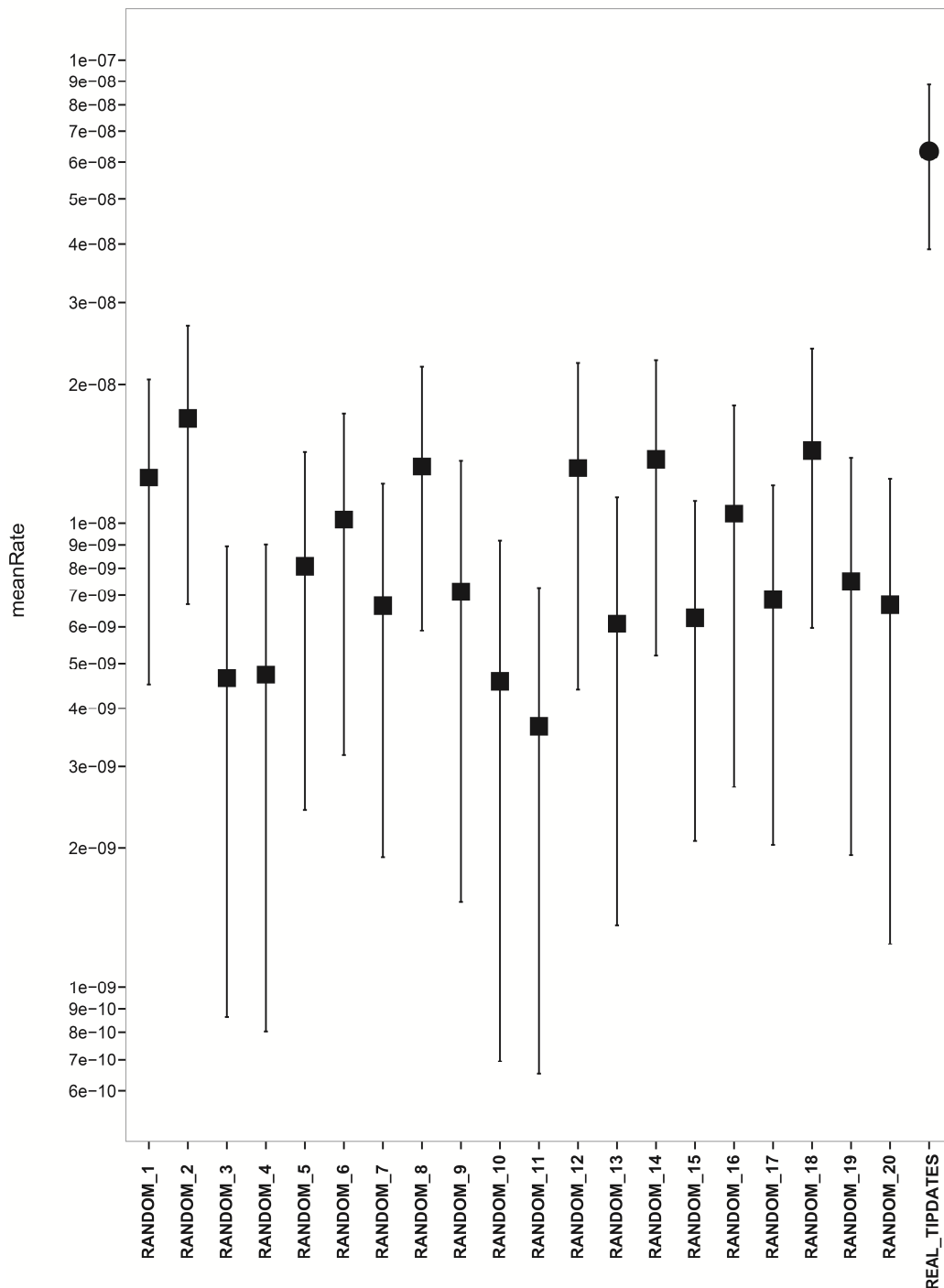
Comparison of substitution rates for randomized and real tipdates
