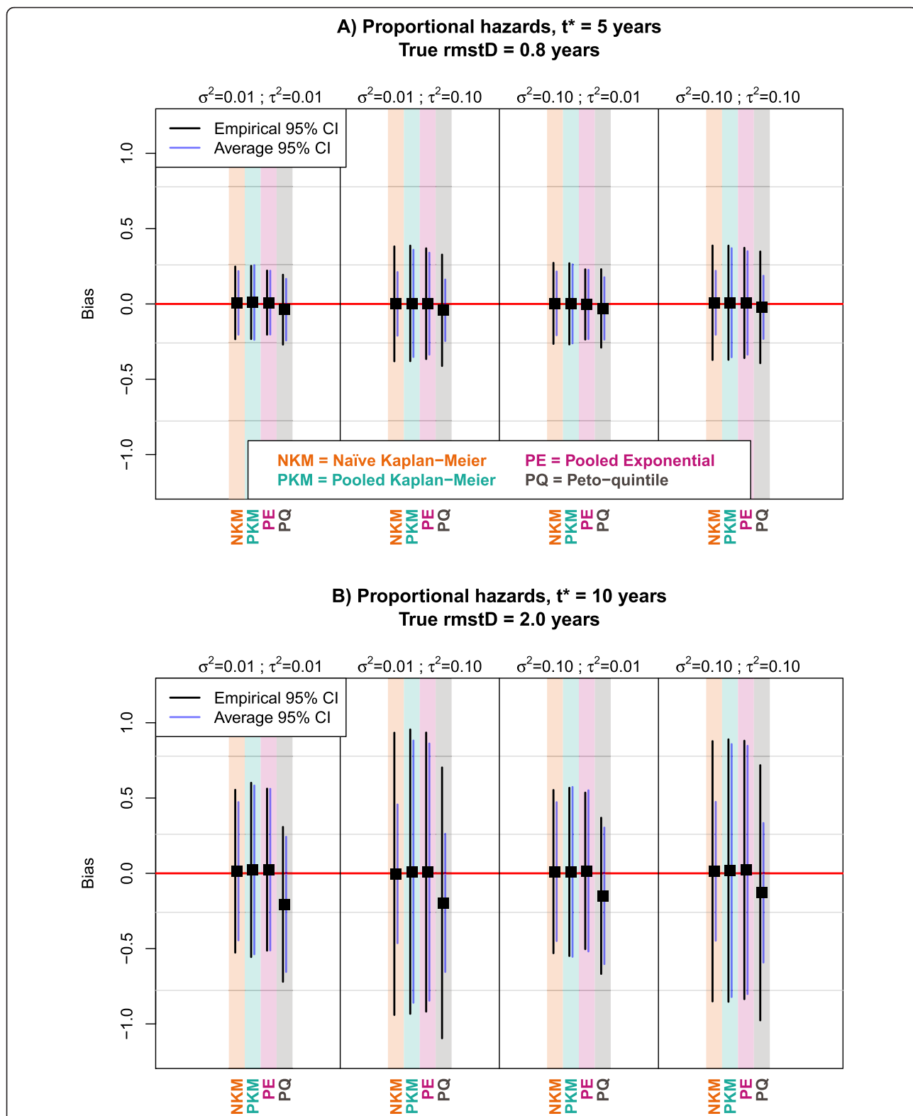
Fig. 1 Graphical comparison at 5 years (panel a ) and at 10 years (panel b ) of methods in terms of bias, empirical and average standard error with proportional hazards; 5 trials and 200 patients per trial; \beta = -0.7 . Black squares represent the average bias of the rmstD estimated by each method for a particular scenario. Black and purple vertical lines represent the 95 % confidence intervals of the bias based on respectively the empirical and average standard errors. The horizontal red line indicates the absence of bias in the rmstD estimation. \beta : Size of treatment effect ( =\log(HR) ); \sigma^2 : baseline hazard heterogeneity; \tau^2 : treatment effect heterogeneity; CI: Confidence interval; rmstD: difference in restricted mean survival time
